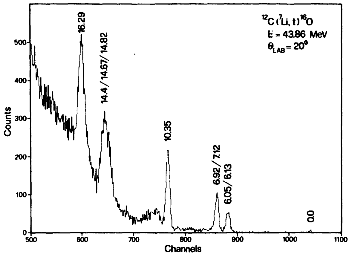
Fig. 8 - Spectrum of the triton emitted in the ^{12}\text{C}(^7\text{Li}, t)^{16}\text{O} reaction at 43.86 MeV incident energy (see text)
