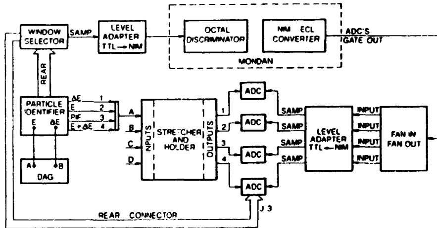
Fig. 6 - Simplified chain for identifier-Mondan connection (see text)
