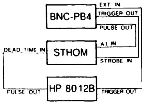
Fig. 5 - Simplified chain for holding test
