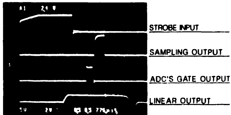
Fig. 7 - Photo of the timing of the 4 most significant pulses from the chain in fig. 6
