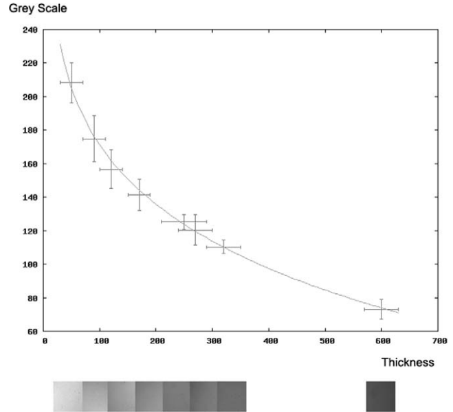
Figure 2. Relation between thickness in \mu\text{m} ( x ) and luminosity in gray scale ( y ).
