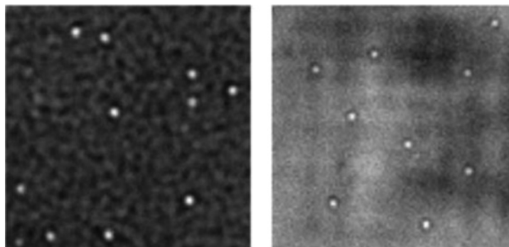
Figure 6: An example readout from an interference reflectance imaging sensor (SP-IRIS) when the substrate is dry (left, 0.8 NA) or when the substrate is mounted in a microfluidic chamber and immersed in water (right, 0.9 NA). Individual vesicular stomatitis virions are detected as small (about 1–3%) diffraction-limited modulations to a reflected reference field. Small fluctuations in the intensity of the reflected reference field are visible in both images. Displayed regions are about 8 \times 8 microns. Adapted from [39] (Reprinted with permission from [39], Copyright 2016 American Chemical Society).
