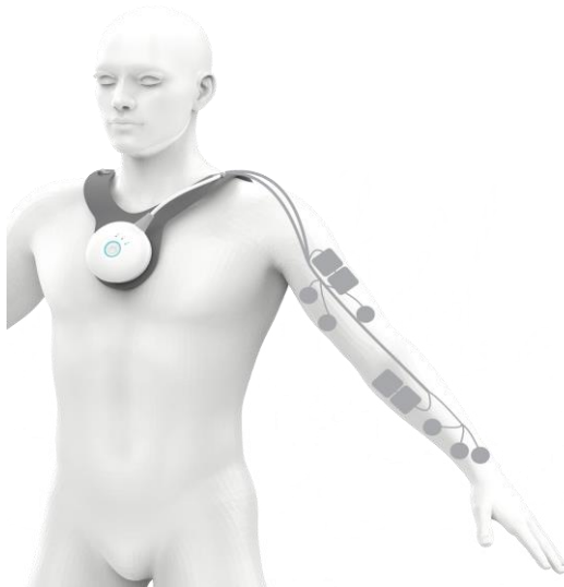
Fig. 5. Final FITFES necklace layout during normal use.
