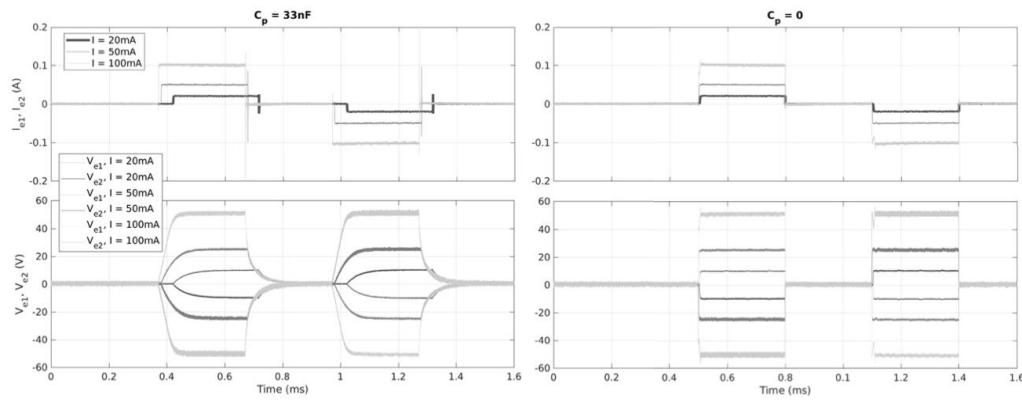
Fig. 10. Currents and voltages of the test circuit given in Fig. 9 at 3 different stimulation levels: 20 mA, 50 mA and 100 mA output, across a pure resistive 1 k \Omega load for 33nF and 0 C_p . The lower traces show the voltage at the terminals and the common mode voltage.
