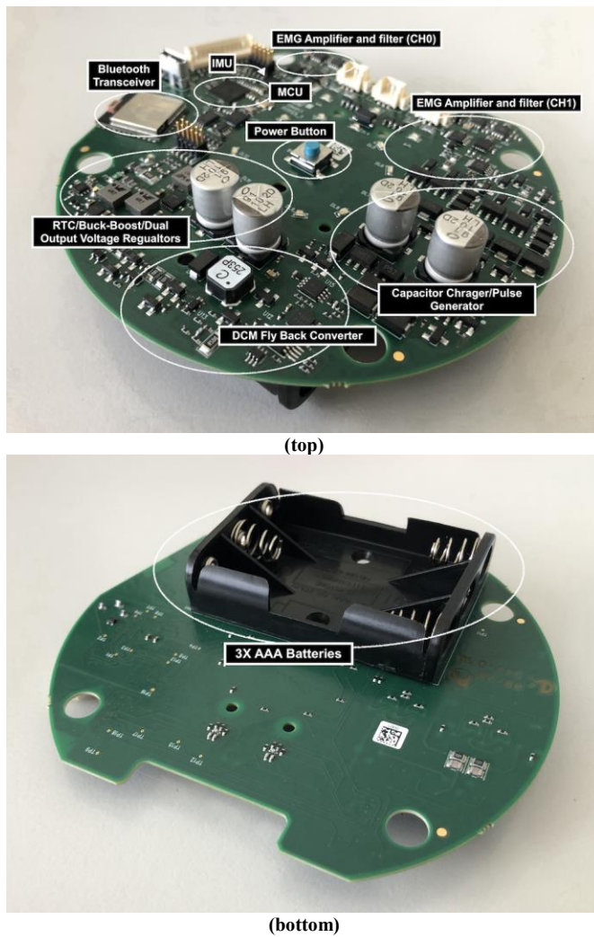
Fig. 8. Photograph of the prototyped printed circuit board, routed to match the mechanical enclosure specifically designed for FITFES, with details on schematic sub-systems placement.
