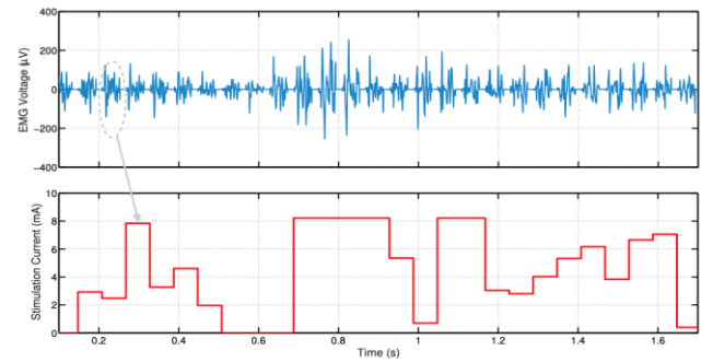
Fig. 12. FITFES real-time stimulation with real EMG data.
