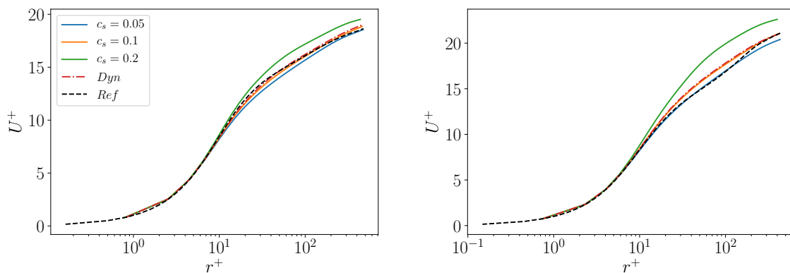
Figure 2. Mean azimuthal (streamwise) velocity profiles in wall units and for the inner cylinder (left) and outer cylinder (right) for selected cases including DNS reference for Rot = 0 .
