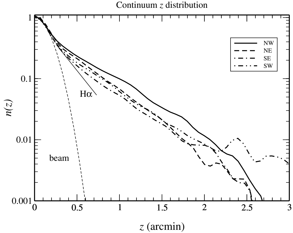
Fig. 9.— Normalised vertical density distributions of the radio continuum halo. The spatial resolution of the observations is indicated. The density distribution of the H \alpha emission as determined by Rand & Heald (priv. comm.) is indicated.
