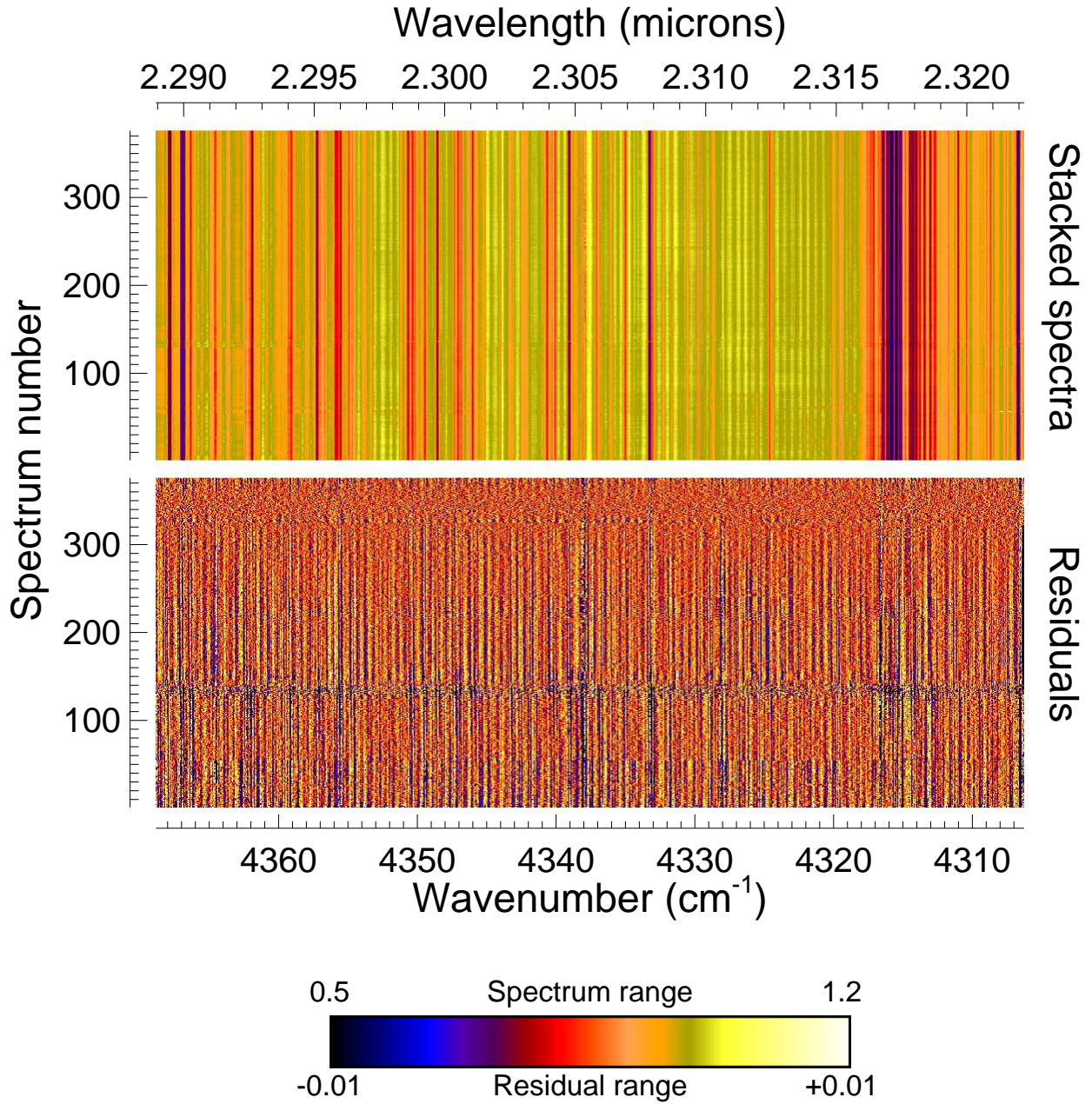
Fig. 4.— Top: Wavelength-calibrated and airmass corrected spectra for echelle order 33 on 26 August 2002. Bottom: Spectral residuals ( r_{\lambda t} ) after digital and Fourier filtering. The color bar shows the range of displayed intensities for the spectra and residuals.
