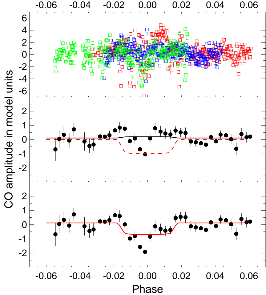
Fig. 6.— Results for the carbon monoxide transit depth for the fiducial model, having cloud tops at 37 mbar. Top: Retrieved CO amplitudes for all 1077 spectra over 3 observed transits (error bars suppressed), red = 19 August, blue = 26 August, green = 2 September. Middle: Data binned by orbital phase (bin width 0.003), with error bars. The black solid line is the least squares fit of the transit curve, having depth -0.09 \pm 0.14 in units of the fiducial model (i.e., no transit CO signal). The red dashed line is a forced fit of transit depth of unity, i.e. CO absorption during transit equal to the fiducial model. Bottom: The recovery of a fake signal input with CO transit depth of unity, and recovered at depth 0.82 \pm 0.14 . Phase=0 is the center of transit.
