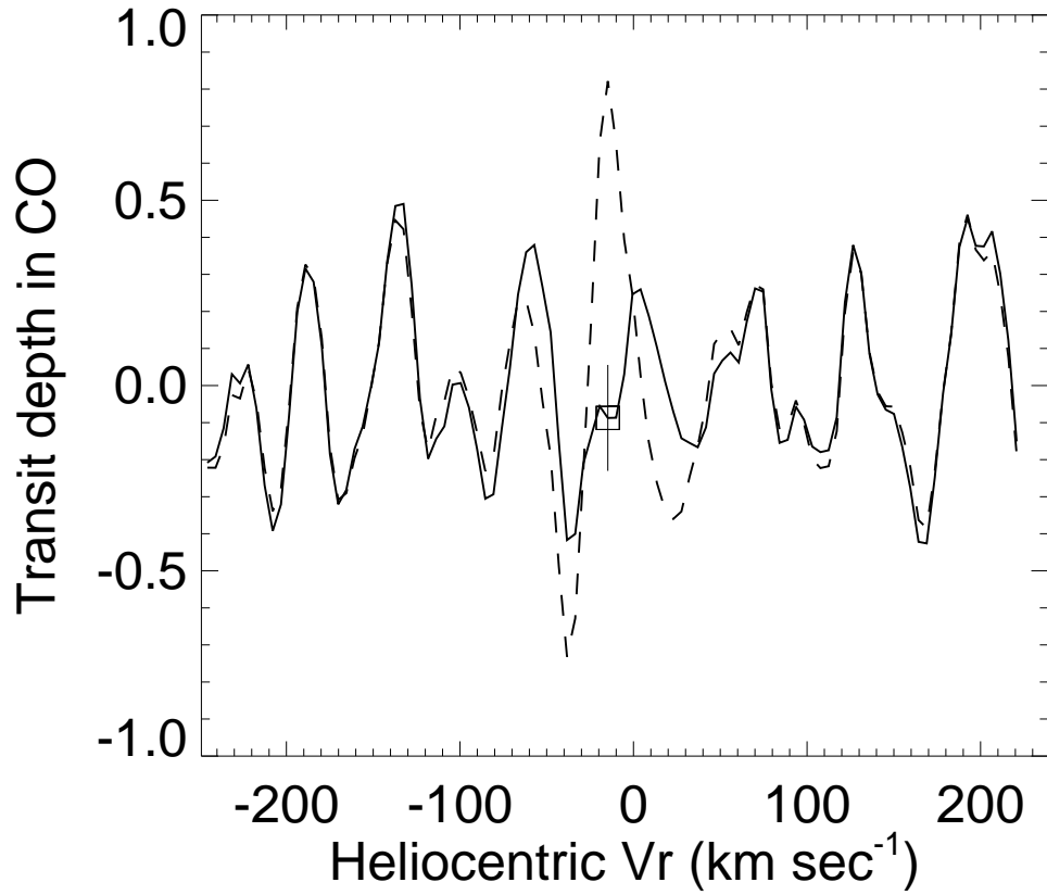
Fig. 7.— Transit depth from our analysis as a function of the heliocentric radial velocity ( V_r ) of the HD 209458 center of mass. The result from the fiducial model is plotted as a single point, with error bar from the fit. The dashed line shows recovery of the fake signal at the correct V_r = -14.8 km sec -1 .
