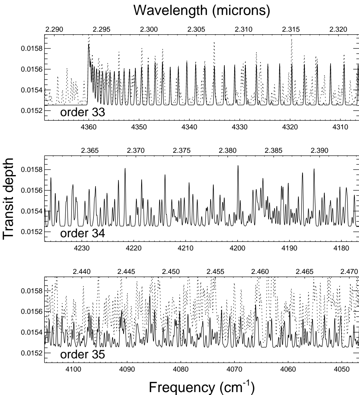
Fig. 1.— Theoretical transit depth for our fiducial model (cloud tops at 37 mbar) in the cases where we consider CO alone (solid line) and CO plus water (dotted line). The template spectra are plotted over the range covered by the 3 NIRSPEC echelle orders that contain CO, and they have been convolved to NIRSPEC resolution.
