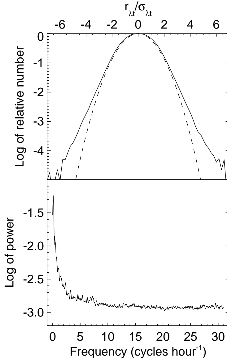
Fig. 5.— Top: distribution of residual values (solid line) compared to a Gaussian normal error distribution (dashed line). The bin size is 0.2 in r_{\lambda t} / \sigma_{\lambda t} . Note log scale used for the ordinate. Bottom: average power spectrum of the residuals, showing the increase in noise at low temporal frequencies. This average power spectrum has been normalized to a total power (area under the curve) = unity.
