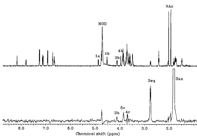
FIG. 1. ^1\text{H} NMR spectrum of sialylated FCHASE-aminophenyl- N -acetyllactosamine. 1a refers to H1 of GlcNAc; 1b , 3b , and 4b denote the H1, H3, and H4 resonances of Gal; and 3eq , 3ax , 4c , and 5c represent Neu5Ac signals. The NOE spectrum (bottom panel) taken from the two-dimensional NOE spectrum shows the NOE from H3 ax of sialic acid to H3 of Gal due to the presence of the Neu5Ac(2-3)Gal linkage in the final product.
