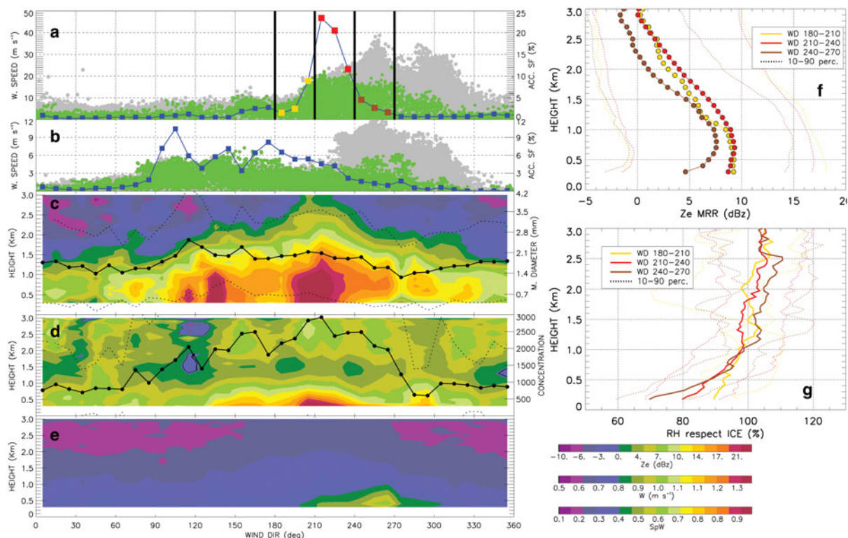
Fig. 8. SF and various MRR product profiles with respect to wind direction (WD). (a) Gray points represent all the AWS Eneide measurements of wind speed ( WS , m s^{-1} ) plotted with respect to WD (deg); green dots correspond to precipitation events highlighted by MRR ( Z_{MRR} > -5 dB). Black line represents the quantity of precipitation calculated with relationship using MRR radar reflectivity measured at 300 m ( SF_{MRR} ), accumulated within each WD bin of 10^\circ width, with respect to total accumulated SF_{MRR} (%). Dots in color refer to the corresponding values for 180^\circ – 210^\circ (yellow), 210^\circ – 240^\circ (red) and 240^\circ – 270^\circ (brown) as in (f, g). (b) As in (a), but referred to the AWS Lucia. (c) Contour plot of the median profiles of radar reflectivity sampled by MRR ( Ze , dBz) within each Eneide WD bin. Average median diameter ( D0 ) and its std dev. for each LPM_{OASI} spectrum within each Eneide WD bin (thick and dotted line, respectively). (d) Contour plot of the mean Doppler velocity profiles sampled by MRR ( W , m s^{-1} ) and averaged for each Eneide WD bin. Average total number of particles and its std dev. detected by LPM_{OASI} data within each Eneide WD bin (thick and dotted line, respectively). (e) Contour plot of the mean spectral width profiles sampled by MRR ( SpW ) averaged within each Eneide WD bin. (f) Median profiles of radar reflectivity sampled by MRR within the Eneide WD bins ( 190^\circ – 210^\circ , 210^\circ – 240^\circ and 240^\circ – 270^\circ ) marked with yellow, red and brown as in (a). Dotted lines represent 10–90 percentiles for each median. (g) As in (f), but referred to median relative humidity with respect to ice ( RHi , %) profiles from radiosounding averaged in the function of 190^\circ – 210^\circ , 210^\circ – 240^\circ and 240^\circ – 270^\circ WD bins (yellow, orange and brown lines, respectively).
