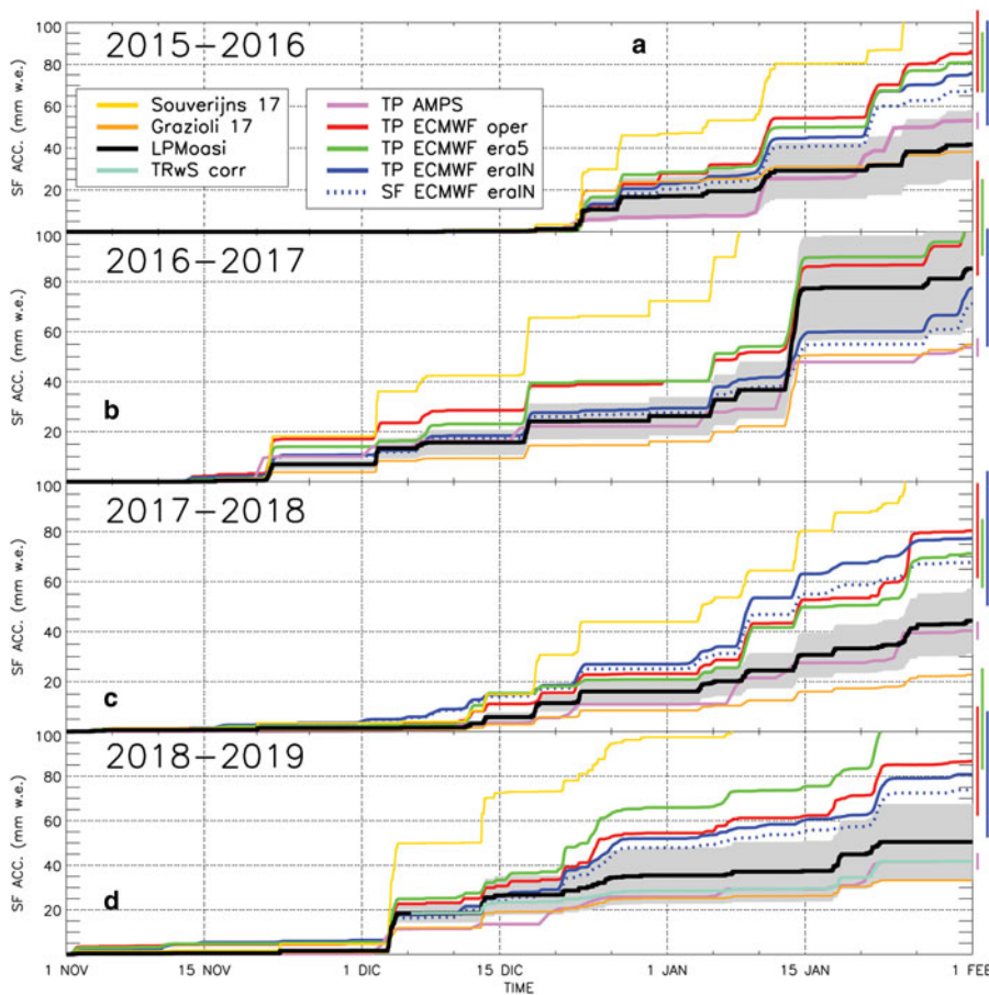
Fig. 5. Time series of accumulated precipitation quantities for the summer campaigns 2015–16, 2016–17, 2017–18 and 2018–19 (a–d, respectively). SF from the MRR reflectivity calculated with Z_e-SF_{RATE} relationship obtained in this paper (see Section 4), highlighted in black line with light gray filled contour representing the associated error. Uncertainties in accumulated values are calculated by adding error propagation in Eqn (5) and variability obtained from the sensitivity analysis, based on the increase/decrease by 20% of velocity/diameter disdrometer data matrix reference bin values. SF from the MRR reflectivity calculated with Z_e-SF_{RATE} relationships defined in Souverijns and others (2017) and Grazioli and others (2017a) are shown in yellow and orange, respectively; whereas the SF calculated from the TRwS snow gauge corrected for false positive, without the 3–5 December 2018 event (see Section 5), is in light blue. Accumulated total precipitation (TP) from ECMWF Operational (OP), ERA5, ERA Interim (ERAIn) and AMPS are shown in red, green blue and violet solid lines, respectively. Vertical bars at the right side and in the same colors represent their associated errors at the last point. Blue dotted line is the ERAIn accumulated value only for the snowfall field.
