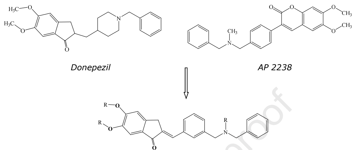
Figure 3 General structure of hybrid compounds bearing a pharmacophoric fragment of donepezil and AP2238.
