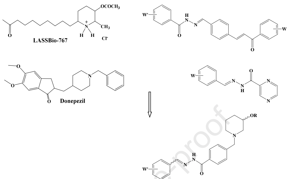
Figure 5 General structure of hybrid N-benzyl-piperidine-aryl-acylhydrazones.
