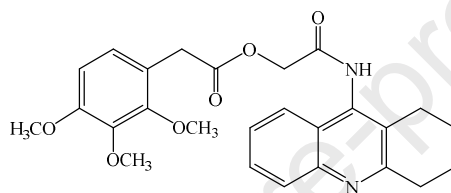
Figure 2 Structure of tacrine derivatives.
