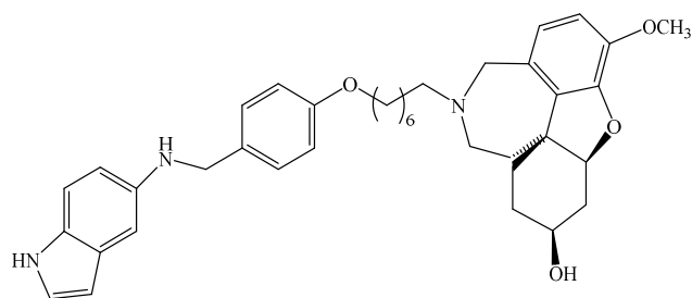
Figure 9 Structure of the most active galantamine-indole.
