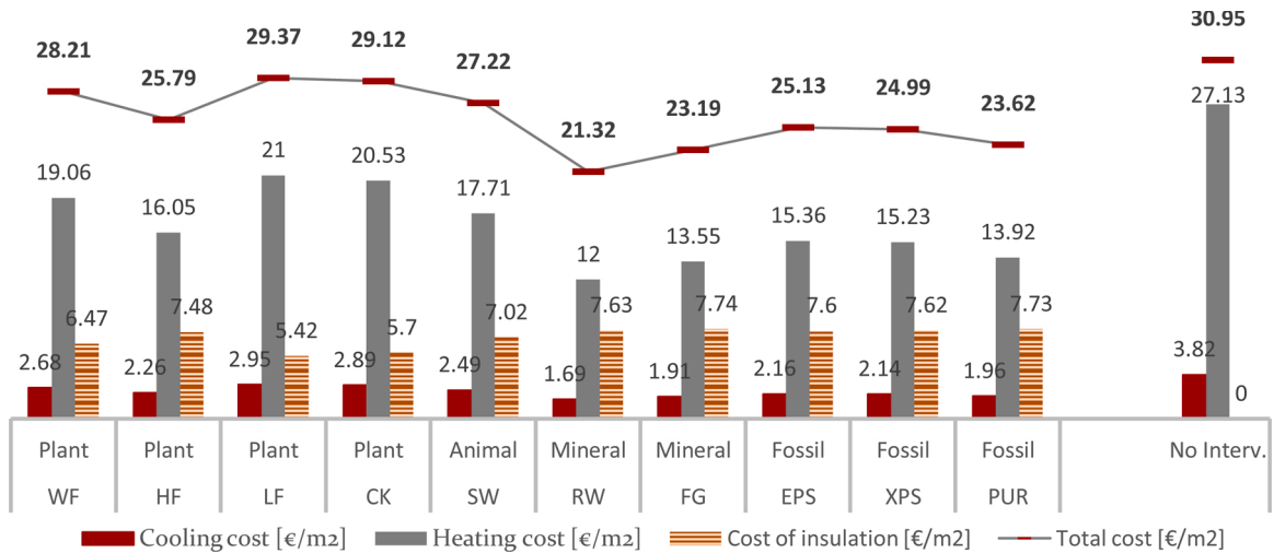
Fig. 4. Estimation results of Cooling cost ( C_c(ins) ), Heating cost ( C_h(ins) ), Cost of insulating material ( C_{ins} ) and Total cost C_t(ins) for all materials under analysis and under the hypothesis of no intervention ( C_c(no-ins) , C_h(no-ins) , C_t(no-ins) ).
