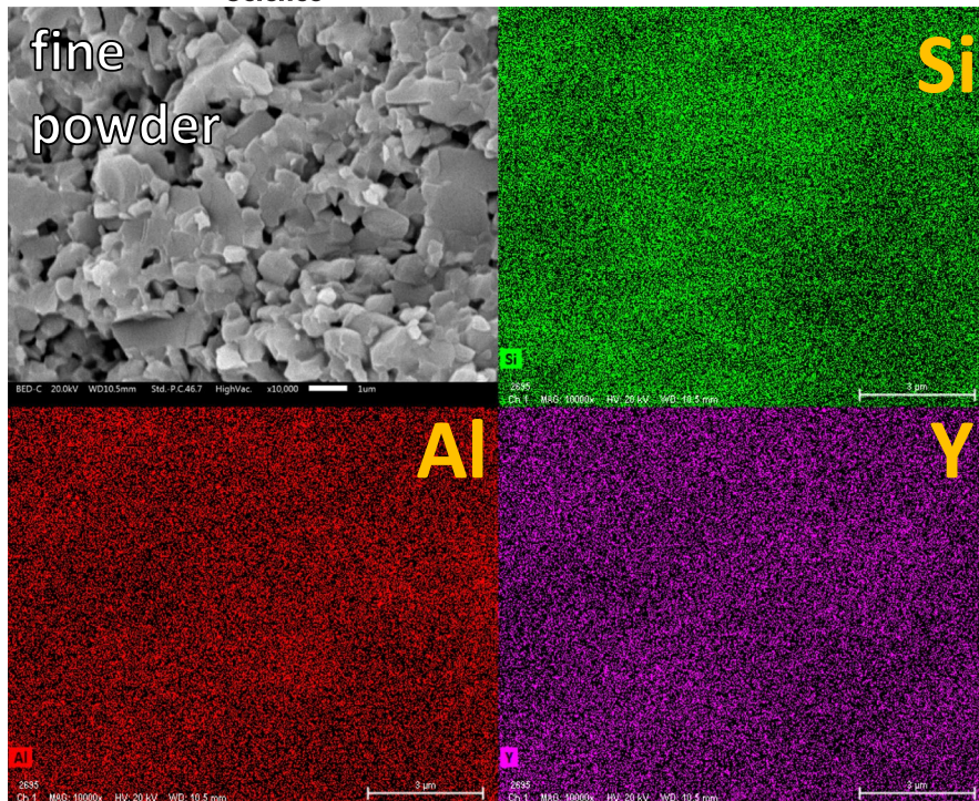
FIGURE 8 Elemental mapping by EDXS analysis on fracture surface of SiC sintered (SPS3) component obtained by 5AY mixture with fine SiC powder
