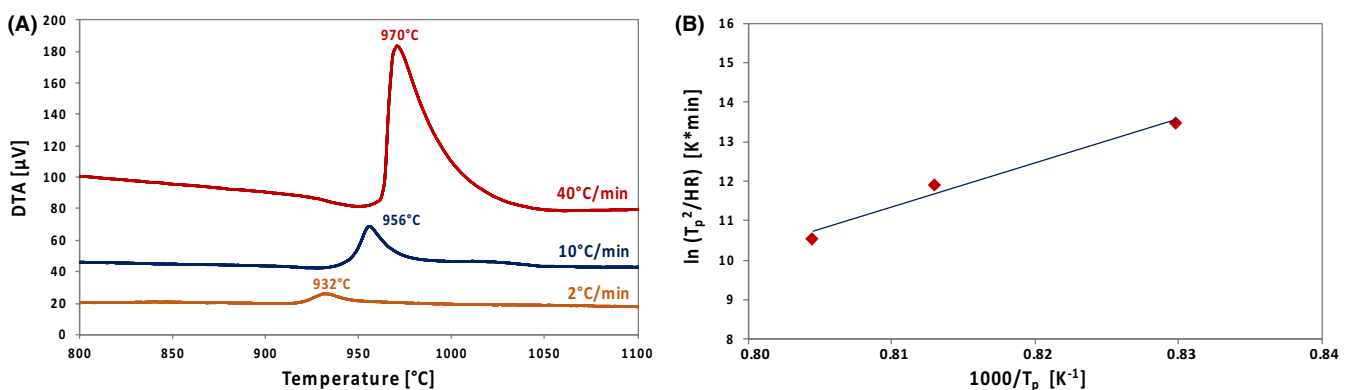
FIGURE 4 DTA on calcined salts (Al 2 O 3 -Y 2 O 3 ) with different heating rates (A); fitting of the experimental points for the determination of YAG crystallization activation energy (B)
