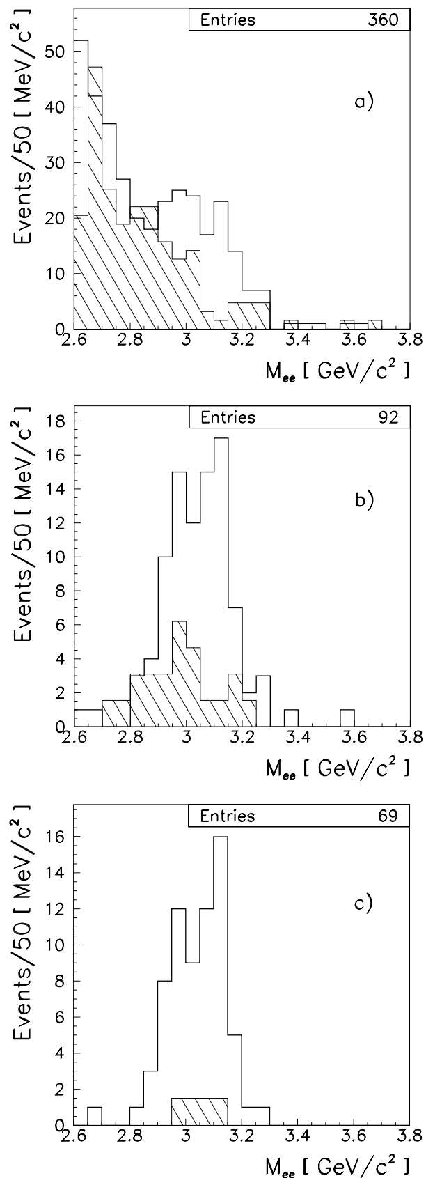
FIG. 1. e^+e^- invariant mass distribution for the events in the resonance region (unshaded) and events in the off-resonance region (shaded). (a) All candidate events; (b) events after kinematic fit; (c) final selected events.
