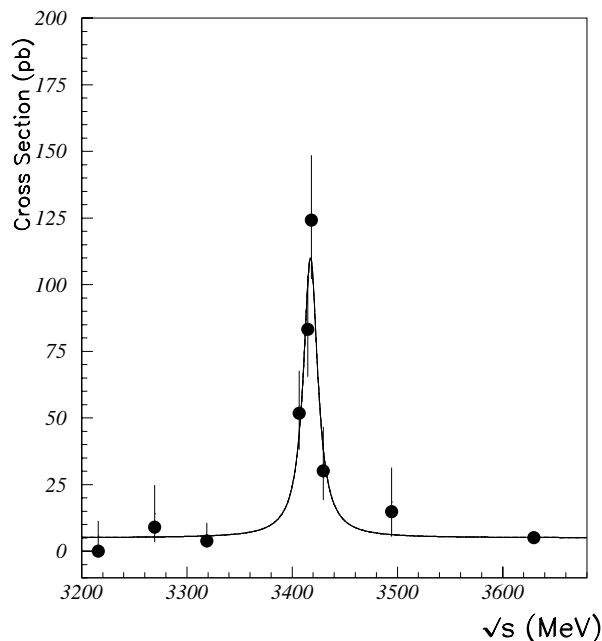
FIG. 2. Measured cross sections and resonance fit as described in the text.
