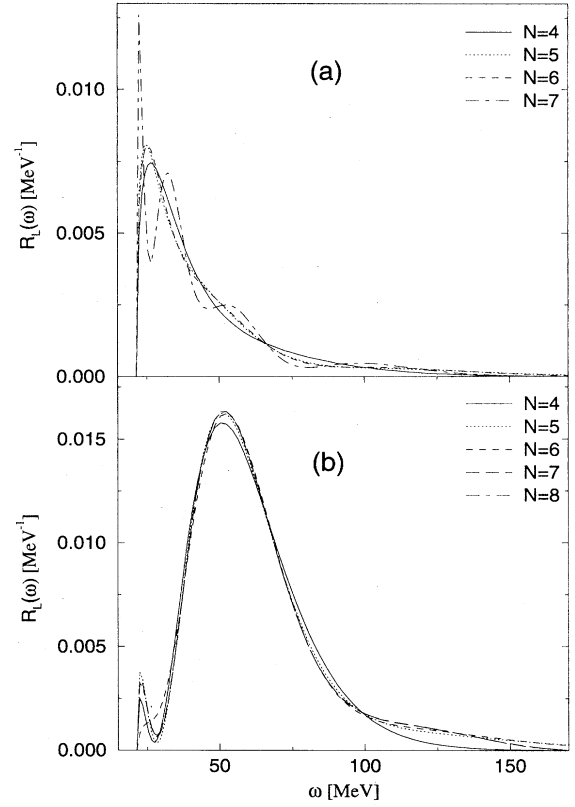
FIG. 3. The longitudinal response function of {}^3\text{He} at |\vec{Q}| = 300 MeV: dependence on the number of basis functions; (a) monopole contribution; (b) sum of all other amplitudes.
