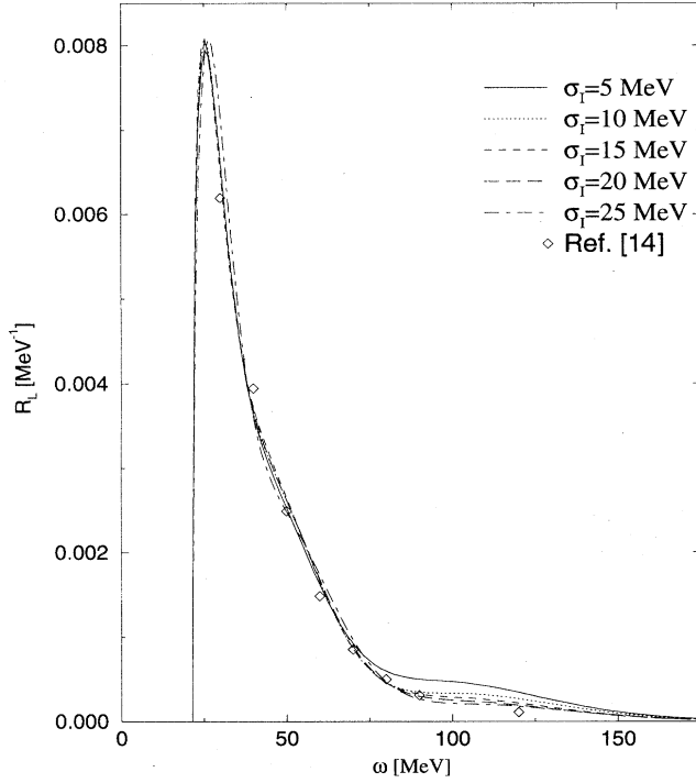
FIG. 2. The monopole contribution to the longitudinal response function of {}^3\text{He} at |\vec{Q}| = 300 MeV/c, for different values of \sigma_I . The results are compared with those obtained in Ref. [14] (diamonds).
