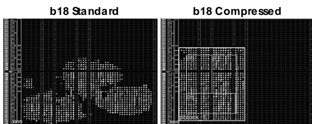
FIGURE 11. Standard (left) and compressed (right) placement solutions for b18 benchmark.
