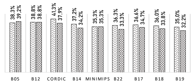
FIGURE 12. Frame Saving without Area constraints (Standard) and with Placement Area Constraints (Constrained).
