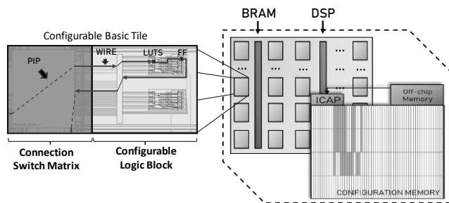
FIGURE 1. An overview of the current FPGA architecture: on the left the basic Tile unit is shown, with detail of the programmable resources and their functions; on the right the two layers fabric is schematized with the configuration memory layer and the programmable resource layer integrated with hardwired resources.
