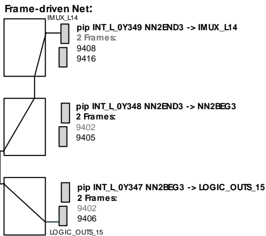
FIGURE 7. The net of the example of Fig. 6 after the FeDRA optimization: by means of the absolute and relative policies 3 frames have been saved.
