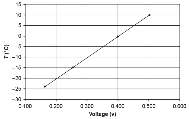
Figure 6. Calibration curve for Vaisala Thermohygrometer.
