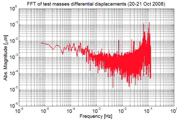
Figure 3. FFT of the relative displacements of the GGG rotating test cylinders, 10 kg each (in the horizontal plane of the lab). Units are in \mu m . Even at low frequencies their separation is below 10^{-8} m , reaching a nanometer at higher frequencies. In the GG space experiment, a weak equivalence principle violation to 10^{-17} would produce a displacement of about 10^{-12} m at orbital frequency
