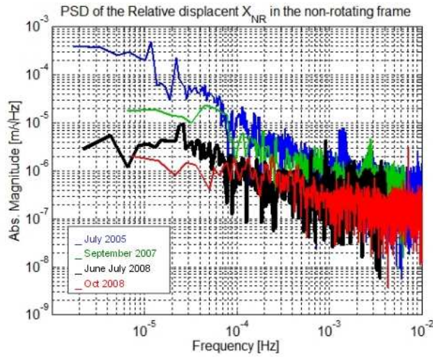
Figure 2. PSD of the relative displacements of the GGG test cylinders showing improvements in sensitivity since 2005. The red curve corresponds to the same 2-day run whose FFT is reported in Figure 3
