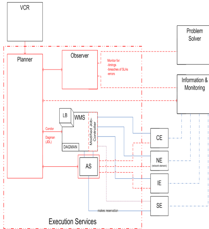
Fig. 2. The GRIDCC Architecture
