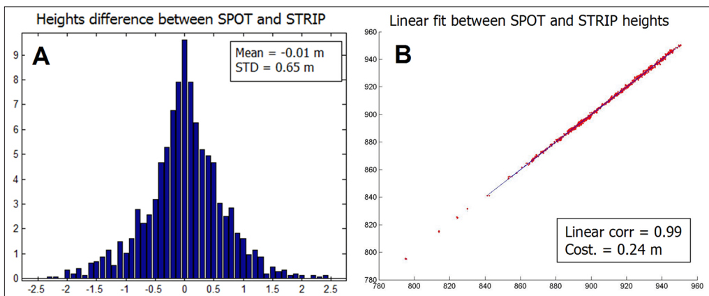
Figure 4 - (A) Histogram of the differences between heights computed by processing Spotlight and Stripmap data. (B) Scatter plot between the heights measurements derived by the two datasets.
