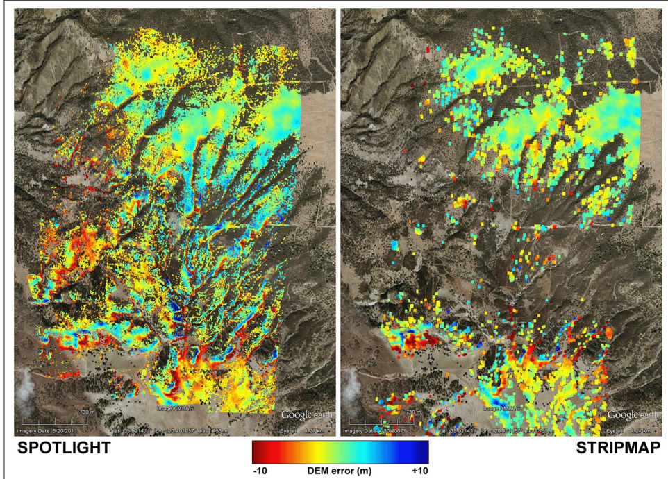
Figure 3 - Height corrections with respect to an SRTM DEM at 1 arcsec computed by using CSK Spotlight (left) and Stripmap (right) data.
