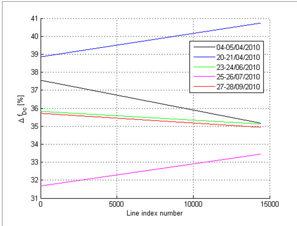
Figure 5 - Trends of the difference between the f_{dc} values of master and slave acquisitions, along azimuth direction. The variation of the Doppler centroid frequency along range direction is instead negligible with respect to the azimuth bandwidth.
