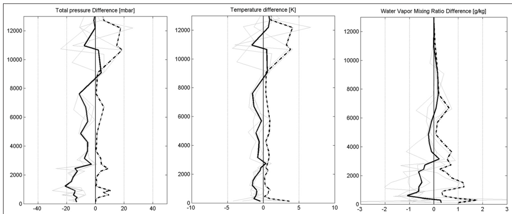
Figure 12 - Comparison between RAMS predictions and RAOBS records (radiosonde 72293 NKX, San Diego). Vertical profiles of (left) total pressure [mbar], (centre) air temperature [K] and (right) water vapor mixing ratio [g/kg] difference between RAMS and RAOBS: solid and dashed bold lines represent mean profile and standard deviation trend along the profile, respectively. Vertical axes represent altitudes in meters.
