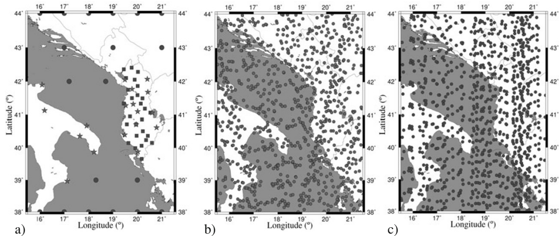
Fig. 1. (a) Location of Italian and Albanian ground magnetic data with 18 vector and scalar magnetic field data points (stars) and 28 scalar magnetic field data points (squares) from 1990 to 2010; 19 synthetic vector data points from IGRF-11 (circles) at 5-year intervals from 1990 to 2005; (b) and (c) are the location of Ørsted (circles) and CHAMP (circles) satellite data used for the SCHA, respectively, from 1999.4 to 2009.4.
