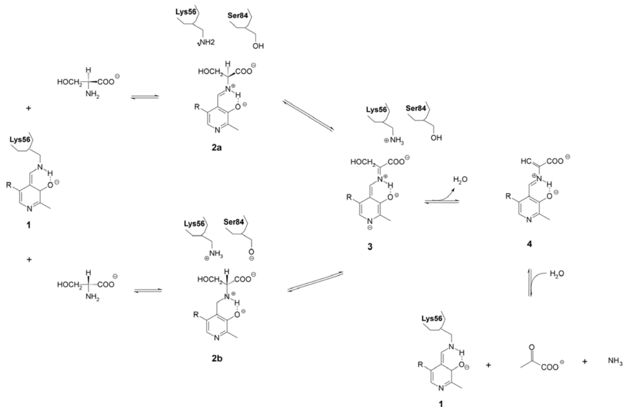
Figure 3. Reaction mechanism of hSR. The deprotonated amino acid substrate reacts with the internal aldimine (1) to give the external aldimine (2a and 2b). External aldimine is deprotonated on the C α by either Lys56, if the incoming amino acid is L-serine, or by Ser84 if the incoming amino acid is D-serine. A quinonoid intermediate (3) has never been observed for serine racemase, but its existence has been postulated based on studies on bacterial alanine racemase (47). The quinonoid intermediate is reformed by either Ser84 or Lys56 and the antipodal amino acid is released with formation of the internal aldimine between Lys56 and PLP. When the hydroxyl group of the quinonoid intermediate is protonated, a β-elimination takes place, with formation of α-aminoacrylate (4), an unstable intermediate that is readily hydrolyzed to ammonia and pyruvate. The protonation can be carried out by either Ser84 or Lys56 depending on the configuration of the incoming amino acid.
