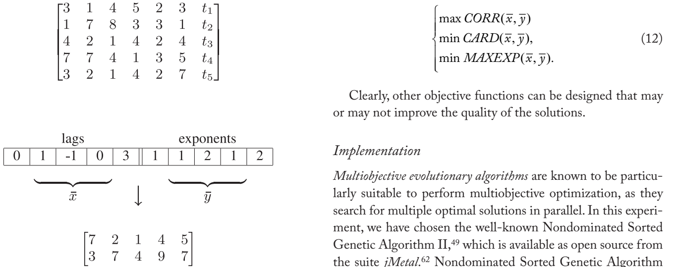
Figure 3. Example of transformation. The original data set (top) is transformed by the pair \bar{x}, \bar{y} (middle) into a lagged data set (bottom), with 1 less feature. There are 3 less instances due to the maximum chosen lag.
