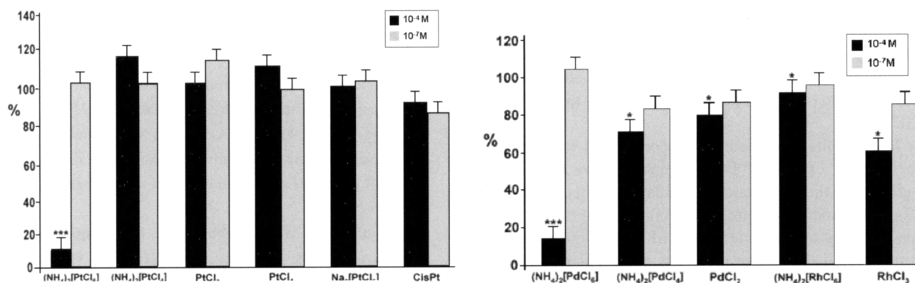
Fig. 4. Percentage (related to the control cultures) of PHA-stimulated TNF- \alpha release from PBMC in presence of 10^{-4} and 10^{-7} M Pd, Pt and Rh compounds. Values are mean \pm S.E.M. ( n = 9 ). TNF- \alpha release in the control cultures is 1319 \pm 133 pg/ml (Man Whitney U test. Significant difference in relation to the control cultures without metal compounds : * p < 0.05 ; *** p < 0.001 ).
