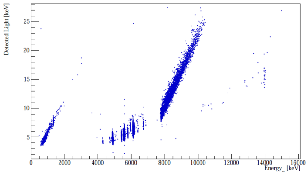
Figure 1. Light-vs-Heat scatter plot corresponding to 19 hours of background measurement with the 57.2 g ^{\text{arch}}\text{PbMoO}_4 scintillating crystal, working as a scintillating bolometer. One can recognize several well separated events distributions caused by different type of particles (see description in text below).
