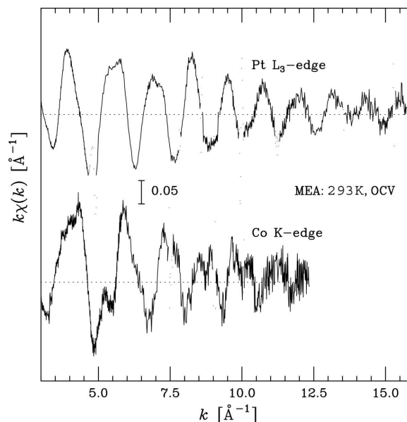
Figure 7 Preliminary in situ measurements on 20% PtCo (1:1)/Vulcan XC-72 cathode electrocatalyst at room temperature. EXAFS signals after Pt L_3 -edge (11564 eV) and Co K -edge (7709 eV). Pt loading: 0.6 \text{ mg cm}^{-2} ; Co loading 0.2 \text{ mg cm}^{-2} . Integration time: 2 s per point. The dotted lines serve as a guide to the eye.
