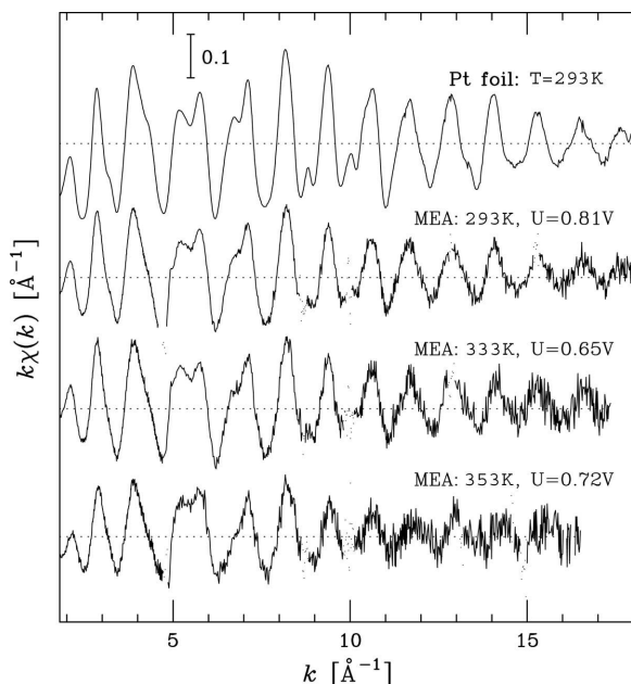
Figure 6 Comparison between EXAFS signals obtained from a Pt foil and in situ MEA (cathode: 20% Pt/Vulcan XC-72 powder, Pt loading 1.0 \text{ mg cm}^{-2} ; anode: 30% Pd/Vulcan XC-72 powder, Pd loading 1.0 \text{ mg cm}^{-2} ) at different temperatures and cell potentials. In situ measurements have been obtained with a beam size of 0.4 \text{ mm} \times 5 \text{ mm} and an integration time per point of 4 s. The dotted lines serve as a guide to the eye.
