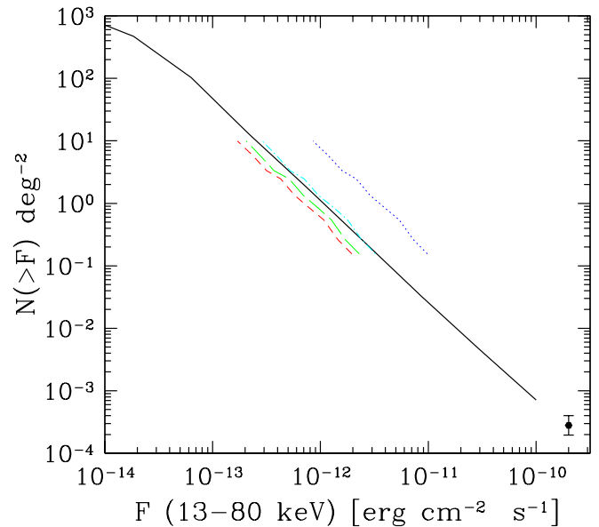
Fig. 7. - The source counts of hard X-ray AGNs contributing to the CXB is shown for the band 13-80 keV, and compared with the HEAO1-A4 data point (Levine et al. 1984). We also show the extrapolation to the 13-80 keV band of the BeppoSAX HELLAS 5-10 keV counts on assuming different absorbing column densities: N_H = 10^{21} cm^{-2} (short-dashed line), N_H = 10^{23} cm^{-2} (long-dashed line), N_H = 10^{23.5} cm^{-2} (dot-dashed line), N_H = 10^{24} cm^{-2} (dotted line)
