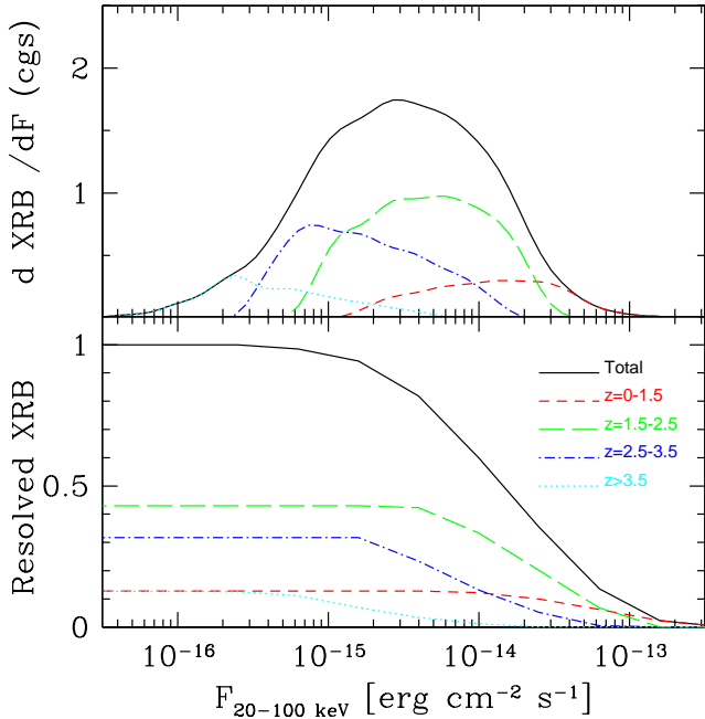
Fig. 6. - Top panel. The 20-100 keV flux distribution of AGNs contributing to the CXB at 30 keV for different bins of redshift (see labels in the bottom panel). Bottom panel. The fraction of the CXB contributed by sources with brighter than the value in abscissa, for the different redshift shells.
