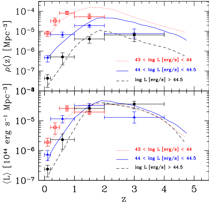
Fig. 8. - Top: The evolution of the number density of X-ray AGNs in three bins of luminosity (in units of erg/s, in the band 2-10 keV): 43 < \log L_X < 44 (dotted line), 44 < \log L_X < 44.5 (solid line), 44.5 < \log L_X (dashed line). The data for the above luminosity bins (squares, triangles, and circles, respectively) are taken from Fiore et al. (2003). Bottom: The evolution of the X-ray luminosity density for the same luminosity bins.
