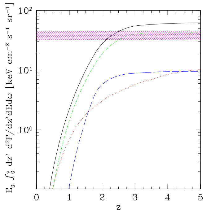
Fig. 2. - The cumulative contribution (multiplied by the energy E_0 ) to the predicted CXB at E_0 = 30 keV, yielded by sources at progressively larger redshifts. The solid line shows the total CXB produced by sources with all luminosities. The other lines show the contributions of AGNs with luminosities L_x (in units of \text{erg s}^{-1} in the band 2-10 keV) in the ranges 42 < \log L_X < 43.5 (dotted), 43.5 < \log L_X < 44.5 (dot dashed), and 44.5 < \log L_X (long-dashed). The shaded strip is the value 43 \text{ keV cm}^{-2} \text{ s}^{-1} \text{ sr}^{-1} measured by HEAO1-A2 (Gruber et al. 1999).
