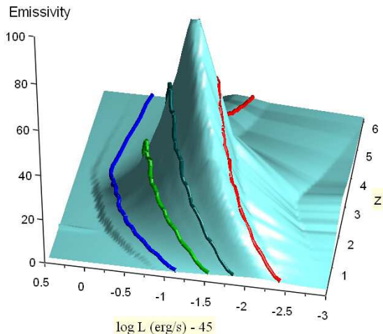
Fig. 1. - The overall X-ray emissivity contributed by AGNs with given X-ray luminosity L_X and redshift z . We also show the evolutionary tracks of the luminosity of AGNs hosted in galaxies with different DM masses corresponding (from left to right) to 10^{13} M_\odot , 10^{12} M_\odot , 2.5 \cdot 10^{11} M_\odot , 5 \cdot 10^{10} M_\odot .
