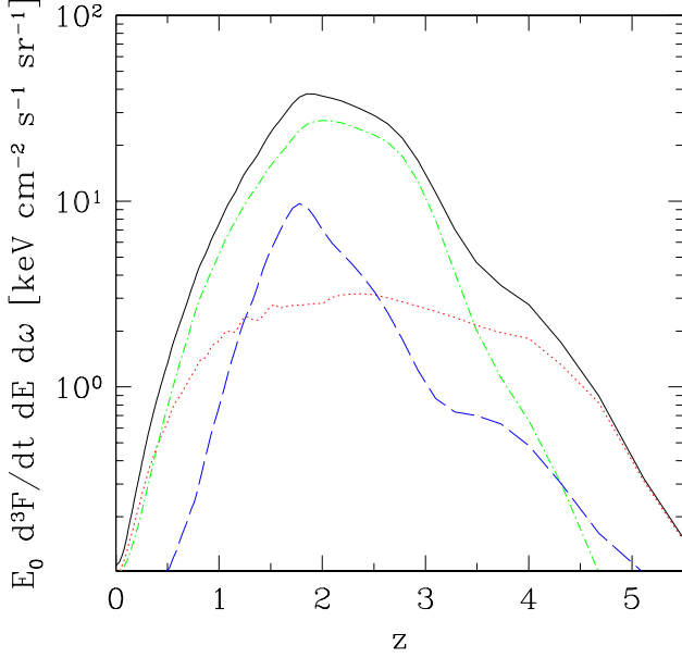
Fig. 3. - It is shown the differential contribution to the predicted CXB at E_0 = 30 keV, for different ranges of luminosity of the contributing sources. Symbols are as in Fig. 2
