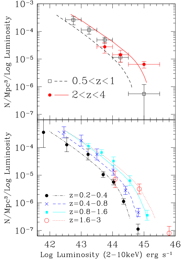
Fig. 9. - The predicted LFs in the energy range 2-10 keV at low redshifts 0.5 < z < 1 (dashed line) and high redshifts 2 < z < 4 (solid line) are compared with observational values derived from the same sample used in Fiore et al. (2003) to derive the densities in Fig. 8.
