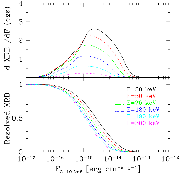
Fig. 5. - Top panel. The flux distribution of AGNs contributing to the CXB at different energies (see labels in the bottom panel). The flux corresponds to the intrinsic emission (corrected for obscuration) in the currently accessible energy band 2-10 keV. Bottom panel. The fraction of the CXB contributed by sources with fluxes larger than the considered value.
