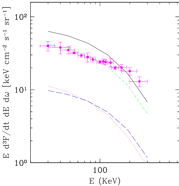
Fig. 4. - The energy spectrum of the predicted CXB for E \geq 30 keV, for different ranges of luminosity of the contributing sources. Symbols are as in Fig. 1. Data are from Gruber et al. (1999).
