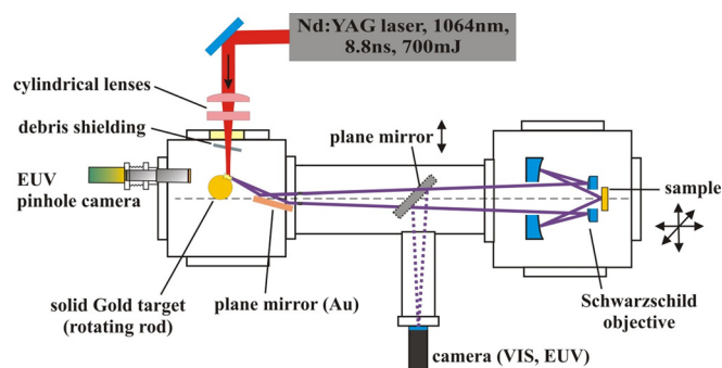
FIG. 1. Sketch of the laser produced plasma facility at Laser-Laboratorium Göttingen e.V. (Germany).
