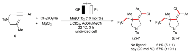
Scheme 3 Electrocatalytic synthesis of chlorotrifluoromethylated pyrrolidines 7 .
