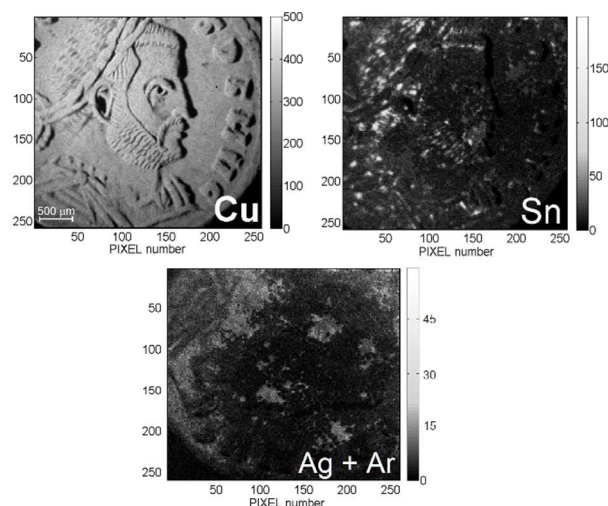
Figure 11. The silvered nummus investigated with the FF-MPIXE technique.
