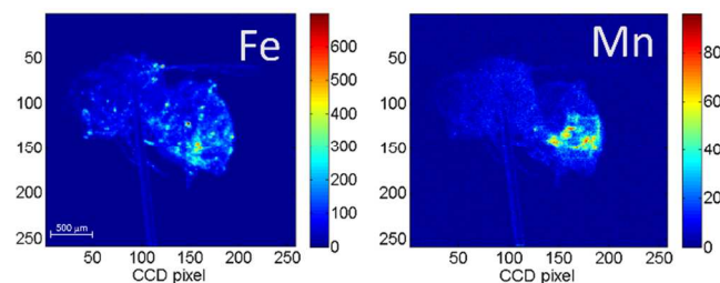
Figure 8. The elemental map of Fe and Mn taken with sample tilted on the back side.
