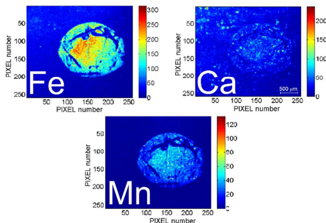
Figure 10. The Nasca sample and the elemental maps obtained by the FF-MPIXE technique.
