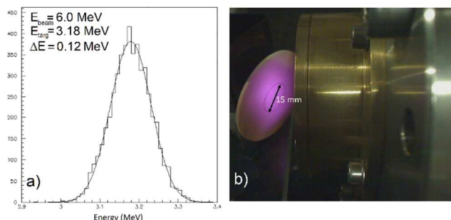
Figure 6. Energy and straggling of proton beam evaluated by a SRIM simulation (a); beam dimension at the sample position (b).
