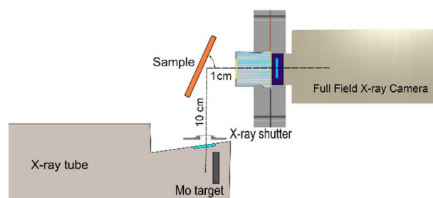
Figure 4. A schematic view of the tabletop FF-XRF instrument.
