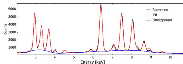
Figure 3. The FF-XRC spectrum processed with the least square fitting module in PyMCA.
