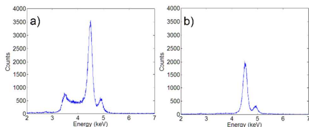
Figure 2. A Ti target measured at a read-out speed of 3 MHz and processed with (a) the previous version of algorithm and (b) the new one.
