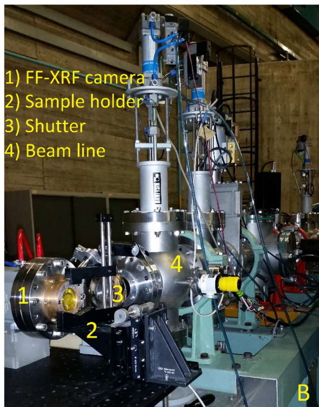
Figure 5. (a) A schematic view of the FF-MPIXE end station (b) and the experimental setup.
