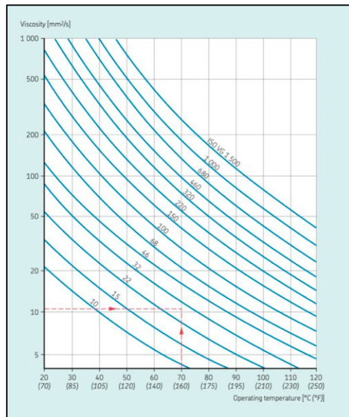
Figure 3: viscosity – temperature diagram [9].
