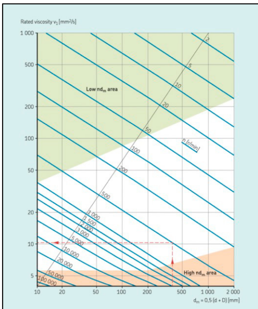
Figure 2: estimation of the rated viscosity \nu_1 [9].
