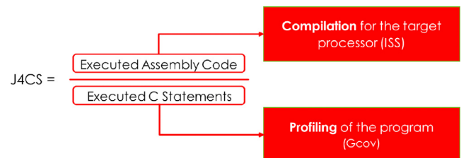
Fig. 3. J4CS evaluation methodology.
