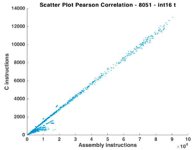
(b) 8051 int16 Corr.
