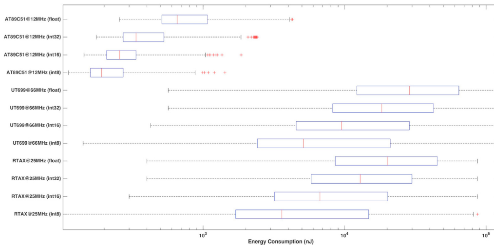
Fig. 11. J4CS-based SW comparison.
