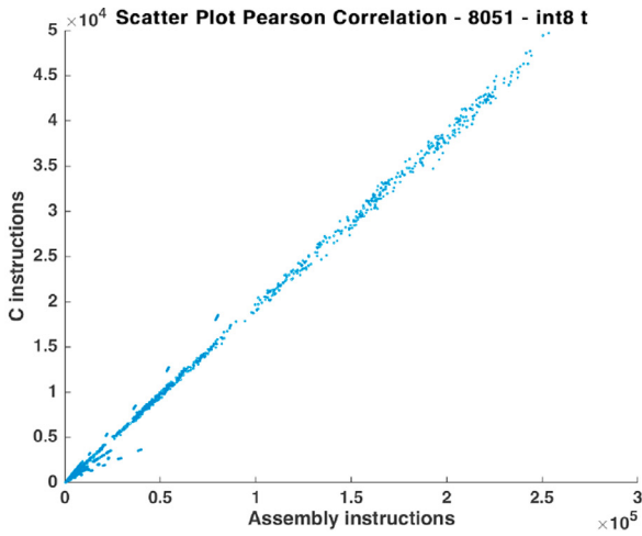
(a) 8051 int8 Corr.
