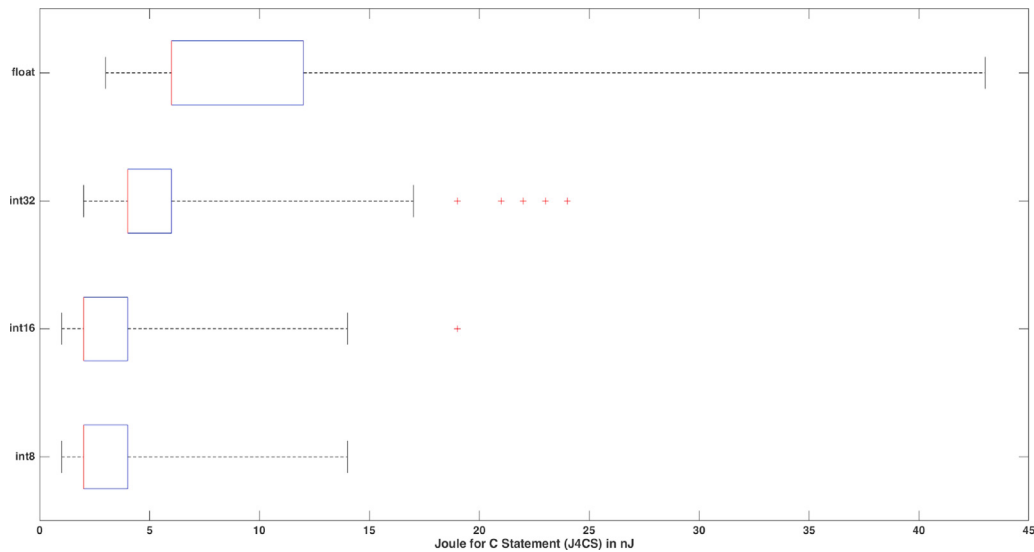
Fig. 10. J4CS BoxPlot results for 8051 (AT89C51 board).
