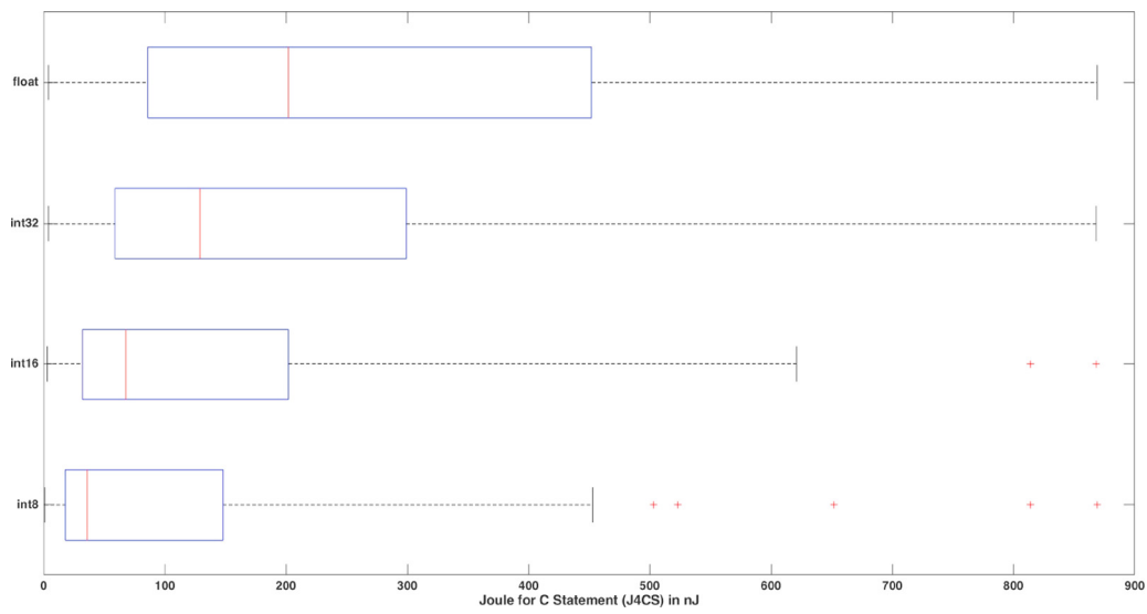
Fig. 8. J4CS BoxPlot results for LEON3 (LEON3FT-RTAX board).
