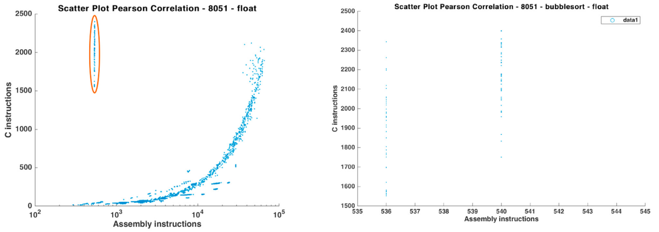
(a) 8051 Float Corr. (Log Scale)
