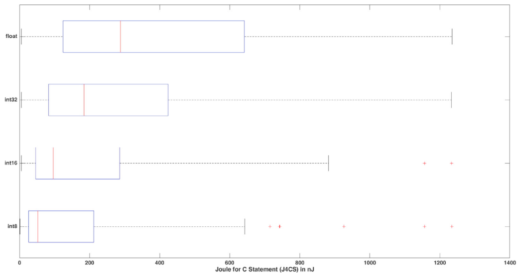
Fig. 9. J4CS BoxPlot results for LEON3 (UT699 board).
