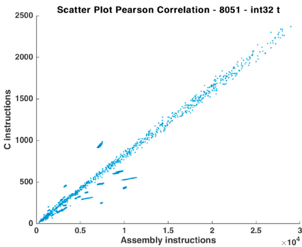
(c) 8051 int32 Corr.
