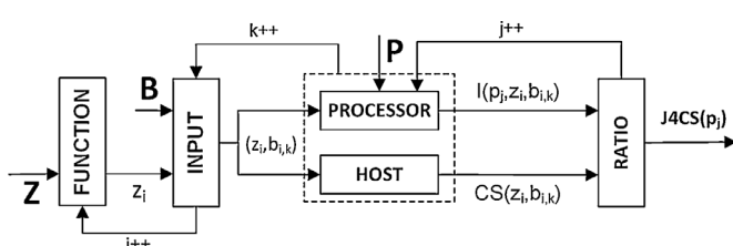
Fig. 2. J4CS evaluation approach.
