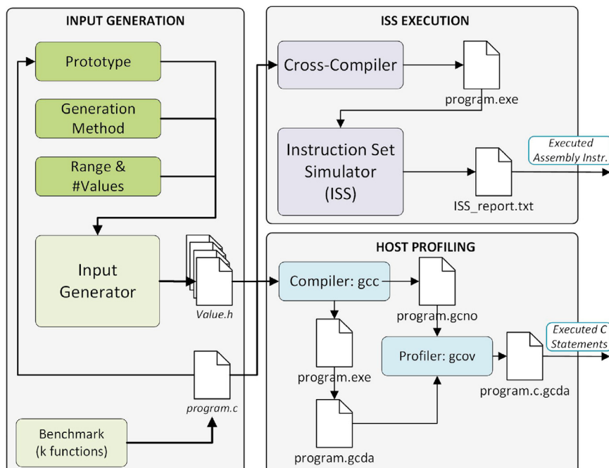
Fig. 4. J4CS evaluation framework.
