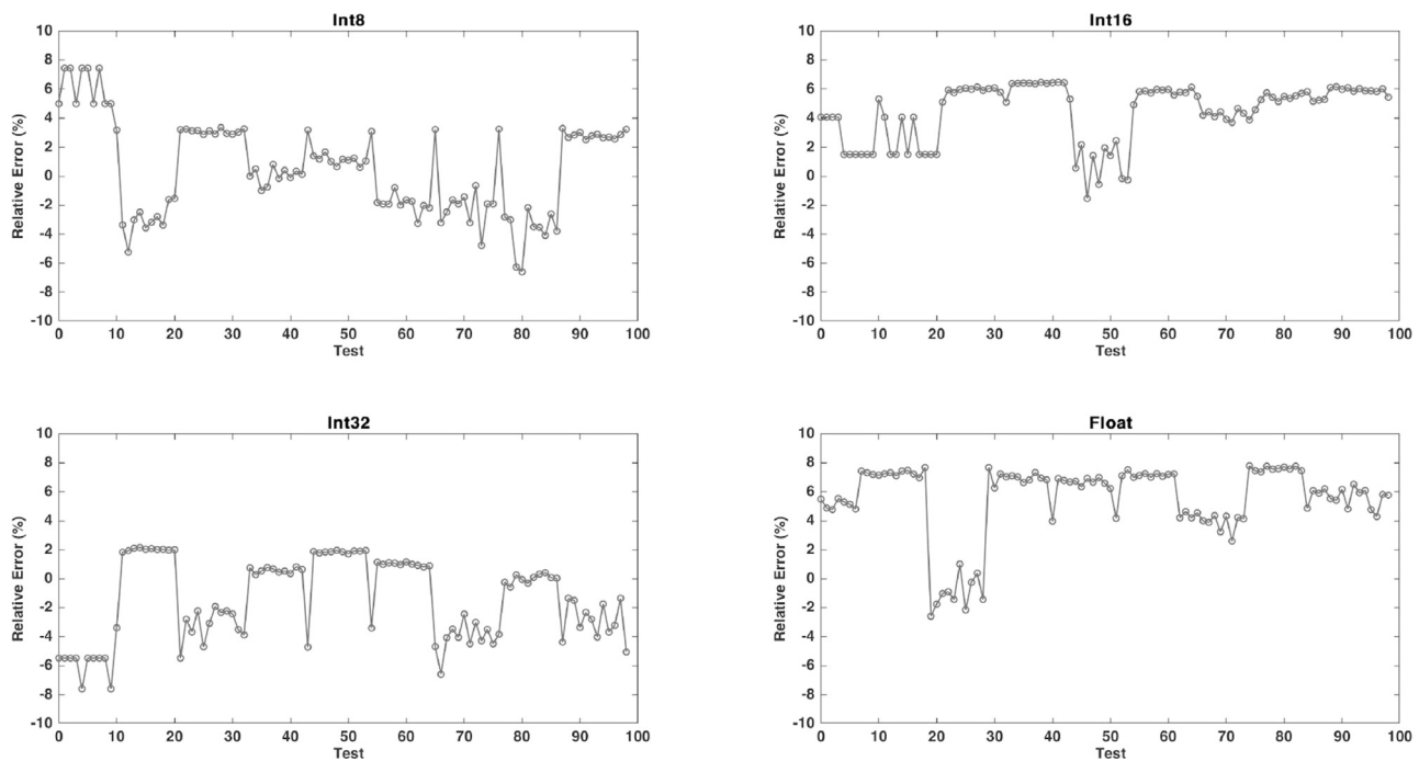
Fig. 13. Relative error plot compared to insertion sort function tests.
