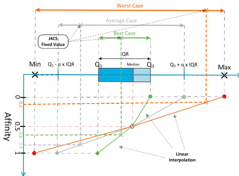
Fig. 12. J4CS-based refinement (considering affinity value).
