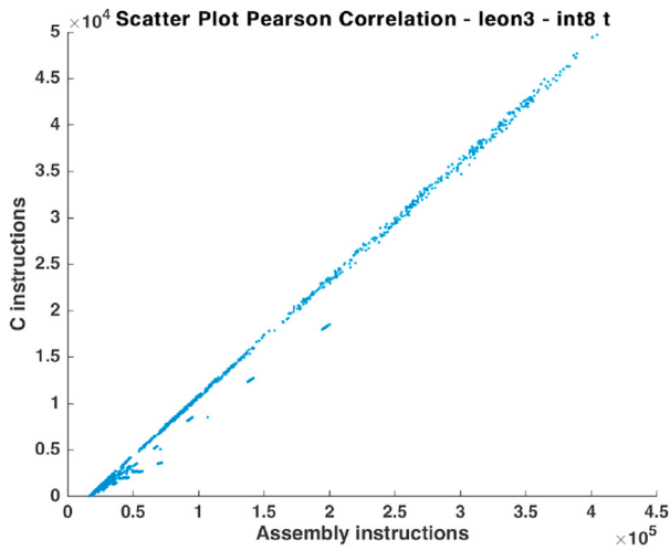
(a) LEON3 int8 Corr.
