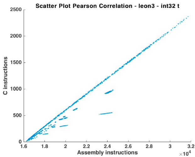
(c) LEON3 int32 Corr.
