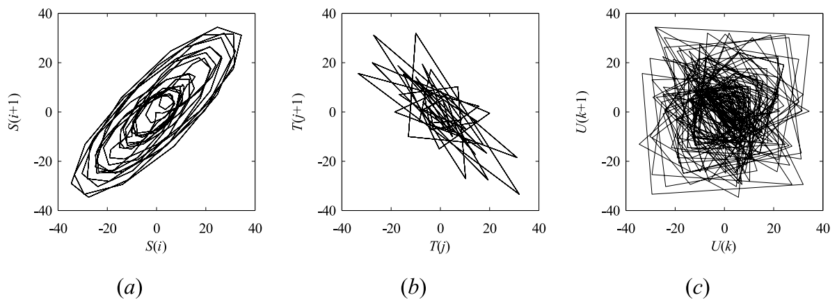
Fig. 4. Delay maps of: (a) S(i) , (b) T(j) , and (c) U(k) .
