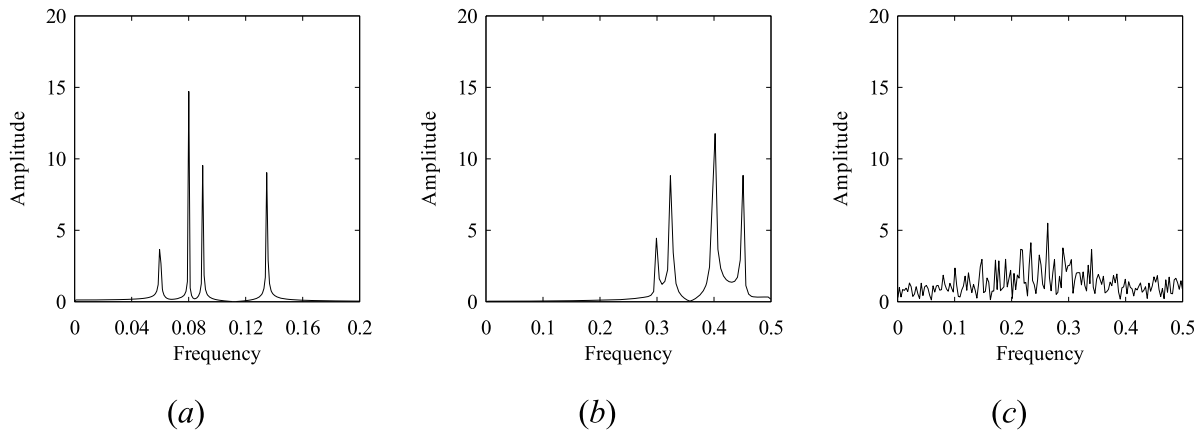
Fig. 3. Frequency domain representations (FFT) of: (a) S(i) , (b) T(j) , and (c) U(k) .
