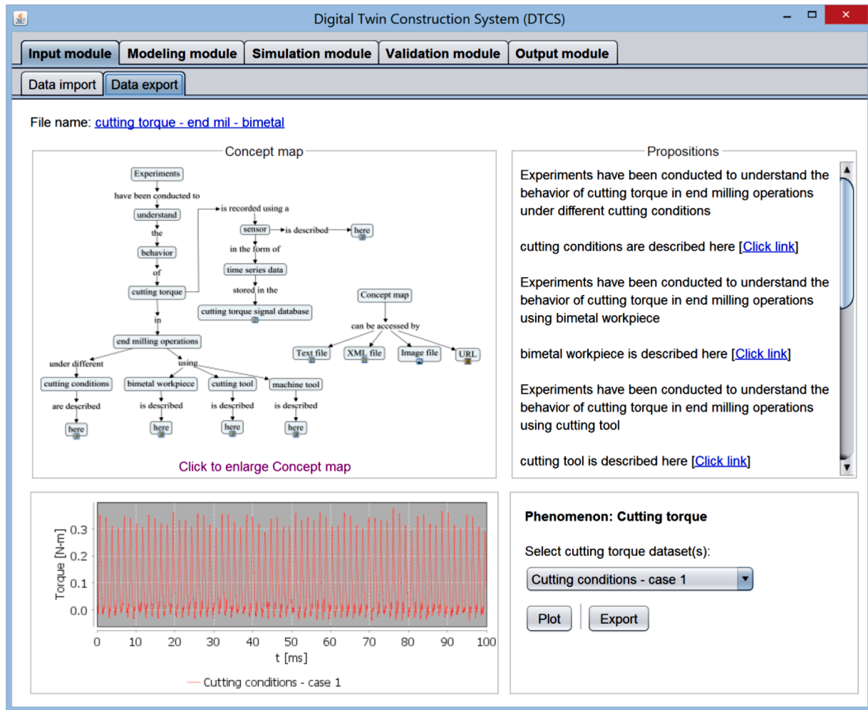
Fig. 13. Screen-print of Data export submodule.
