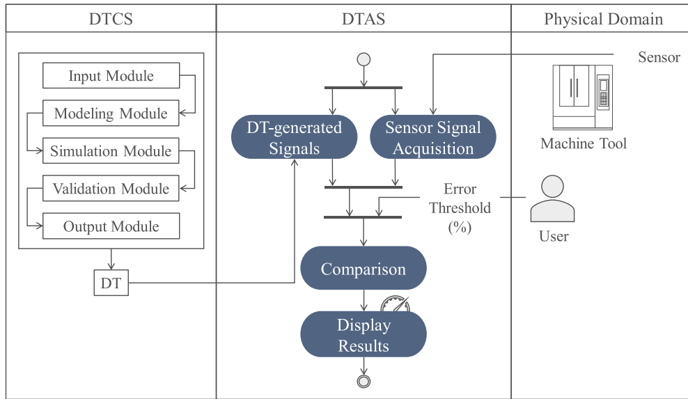
Fig. 11. Modular architecture of the DTAS.
