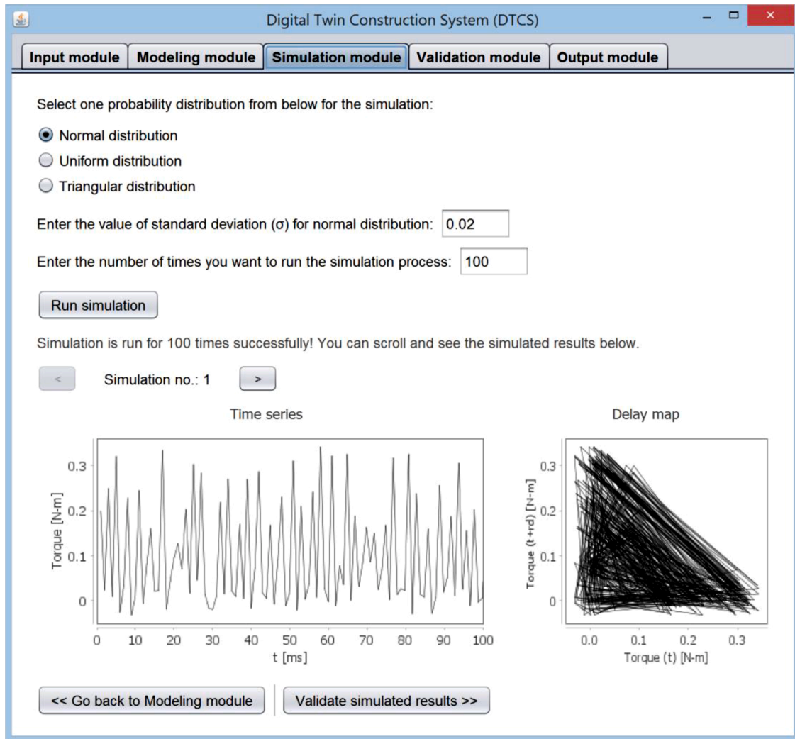
Fig. 15. Screen-print of Simulation module.
