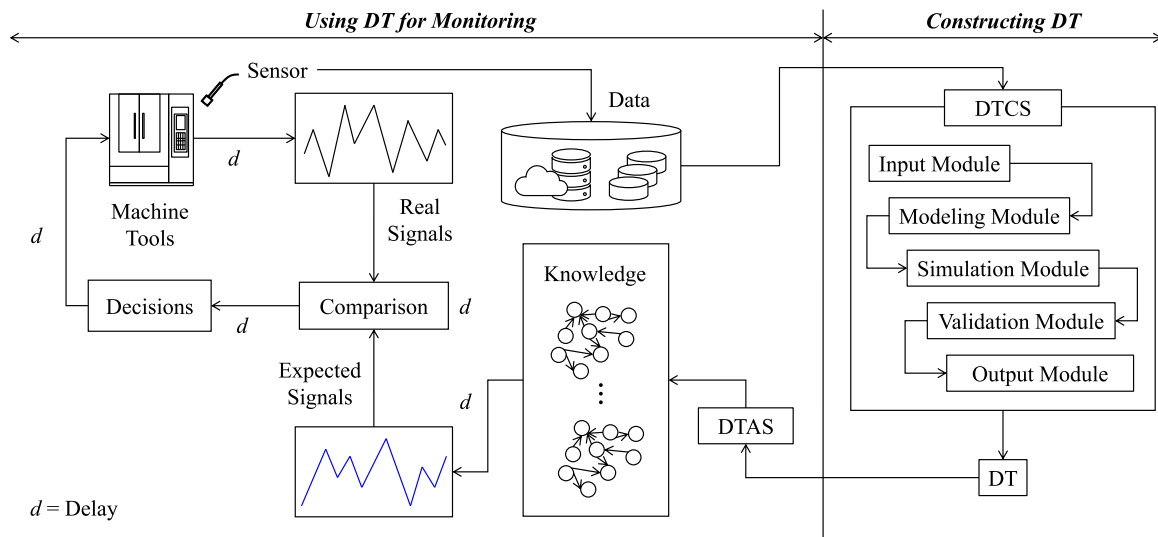
Fig. 5. Construction and use of DT in intelligent machine tools.
