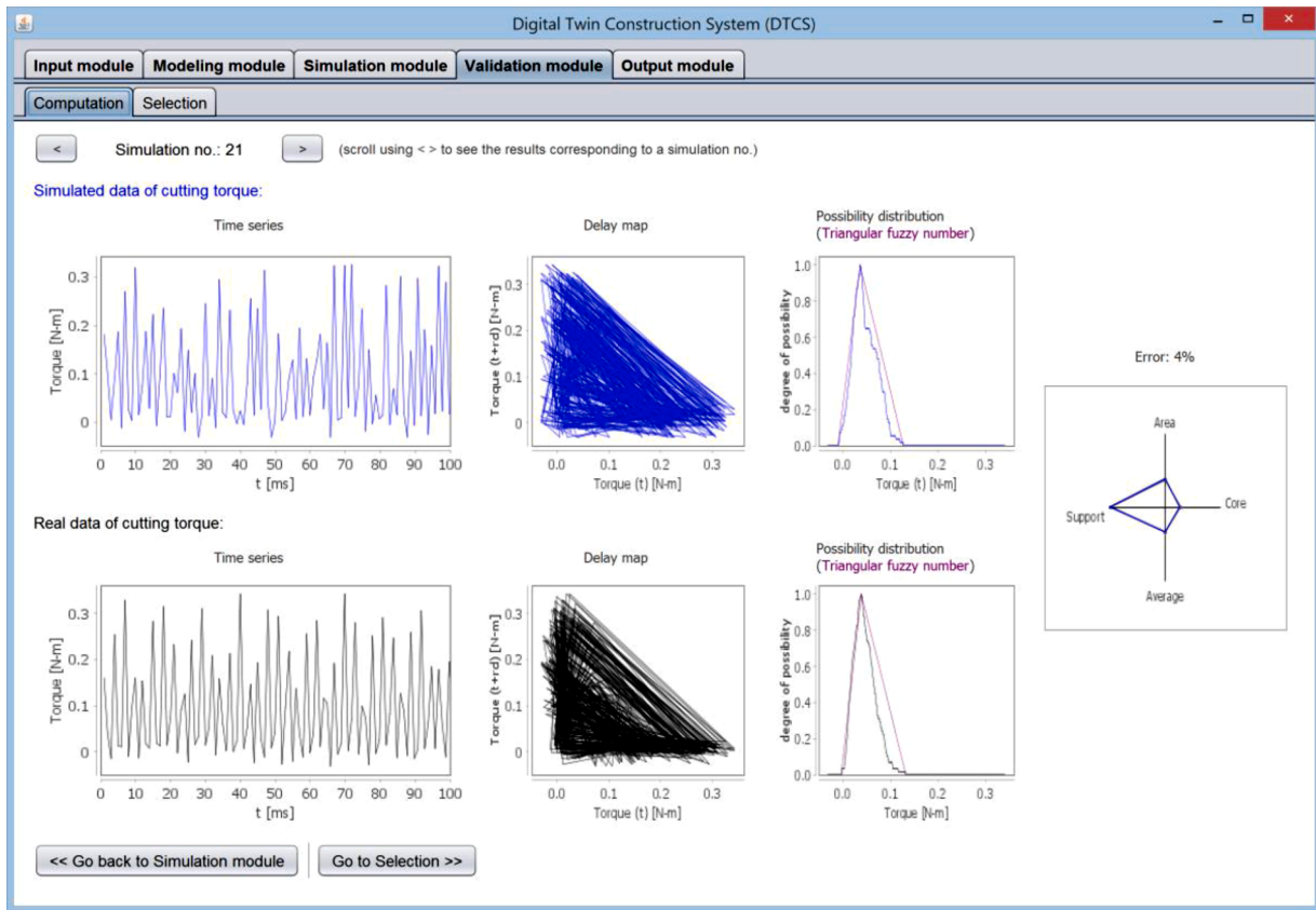
Fig. 16. Screen-print of the Computation submodule.
