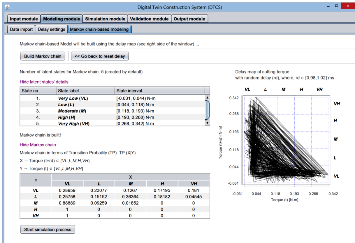
Fig. 14. Screen-print of Modeling module.
