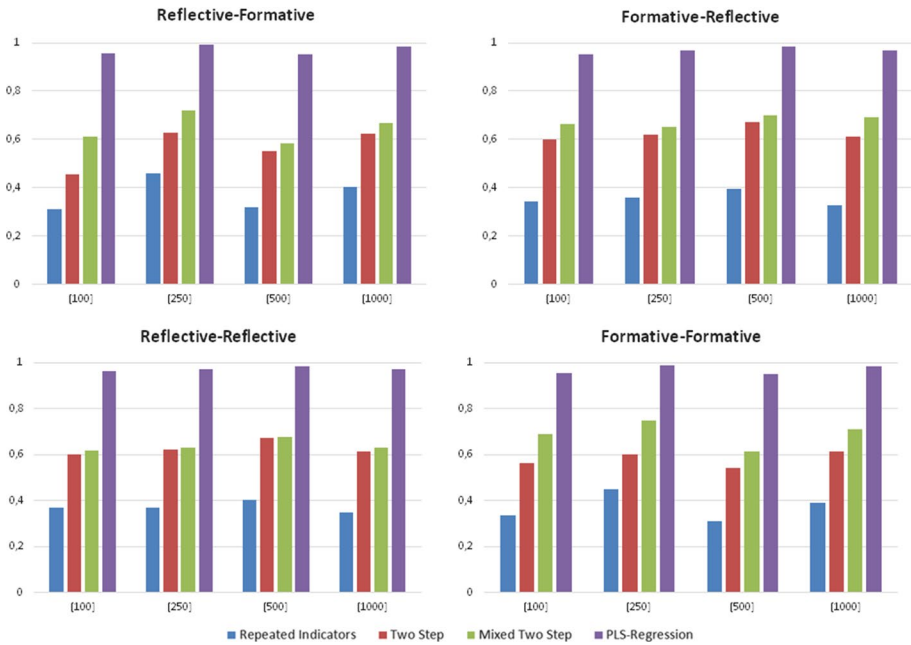
Fig. 6 Community comparison
