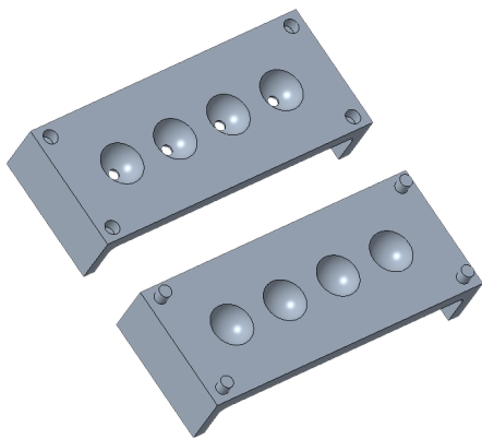
(a) CAD perspective view.
