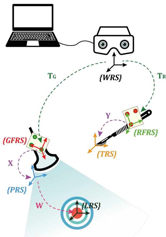
FIGURE 2. Diagram of the component of the integrated system. The diagram shows the respective reference systems and the associated rototranslation matrices.
