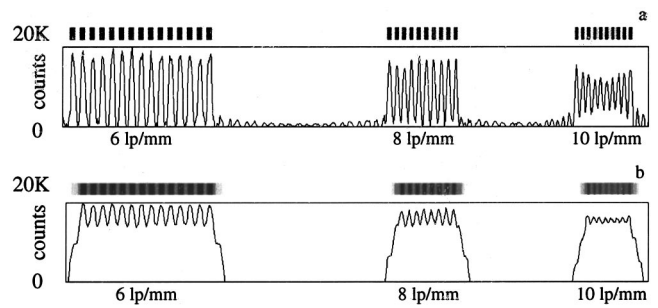
FIG. 3. Images of a bar pattern test object, obtained by scanning the sample with a step (20 μm) smaller than the pixel size (300 μm): (a) the processed image featuring a spatial resolution increase, (b) the raw image.
