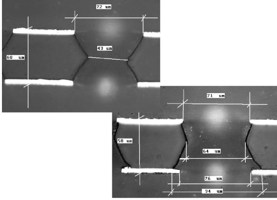
Figure 4. Cross section of first GEM foil (left) and third GEM foil (right) of aged chamber A.
