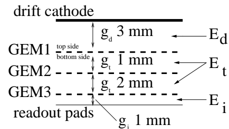
Figure 1. Cross-section of the triple-GEM detector. E_d , E_t and E_i are the drift, transfer and induction fields respectively; g_d , g_t , and g_i are the drift, transfer and induction gaps respectively.
