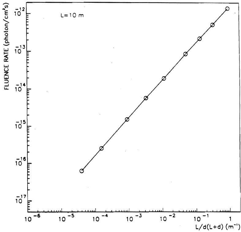
FIG. 3 – Fluence rate per e - /s as a function of L/d(L+d) in the case of a straight section 10 m long operating at 1.33·10 -7 Pa (10 -9 torr). Primary electron energy 510 MeV.
