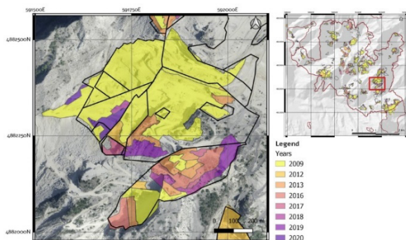
Figure 4. Sample site with yearly detected changes areas (1:5000). Black outlines represent quarries' own properties extents. Background: 2019 orthoimage.
