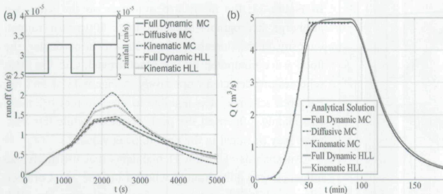
Figure 7 | Comparison of the simulated runoff hydrographs using MacCormack's scheme and the HLL scheme: (a) Test 1, (b) Test 2.
