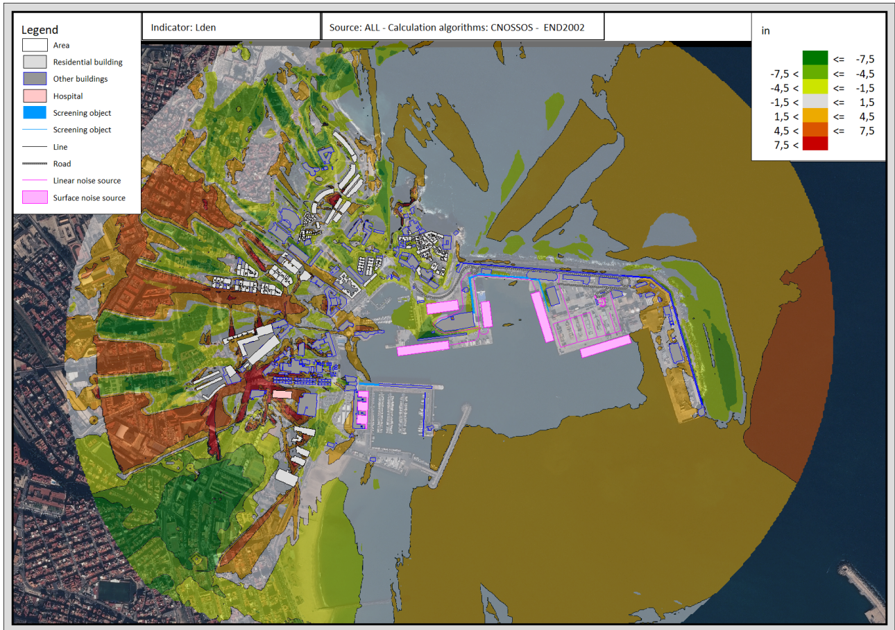
Figure A3: Difference between L_{den} estimation with 2015/996 algorithm and the one of the old Annex II of the END
