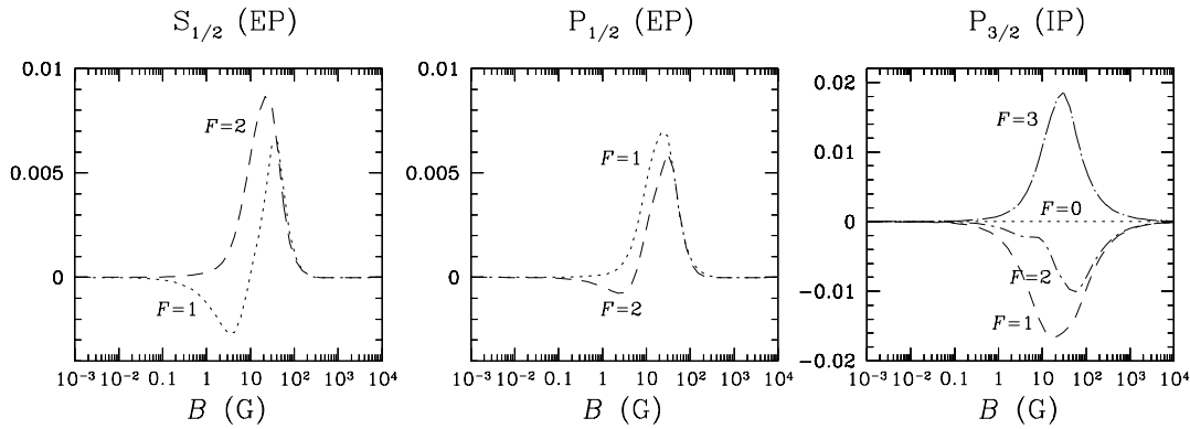
Fig. 2.— Fractional atomic orientation, \sigma_0^1(F) = \rho_0^1(F, F)/\rho_0^0(F, F) , of the three lowest levels of Na I against the magnetic field strength (notice the different range of magnetic strengths with respect to Fig. 1). The scattering geometry and the plasma conditions are the same as in the calculation of Figure 1. These results show that atomic orientation in the levels of D 1 is negligible for fields B \gtrsim 100 G.
