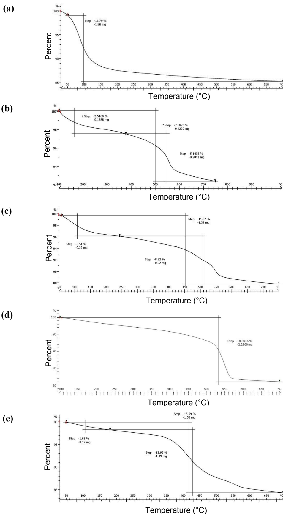
Figure 4: TGA analysis of 15 nm-sized SiNPs; (a) Pristine, (b) C3-COOH, (c) C11-COOH, (d) NH 2 , (e) PEG-modified SiNPs
