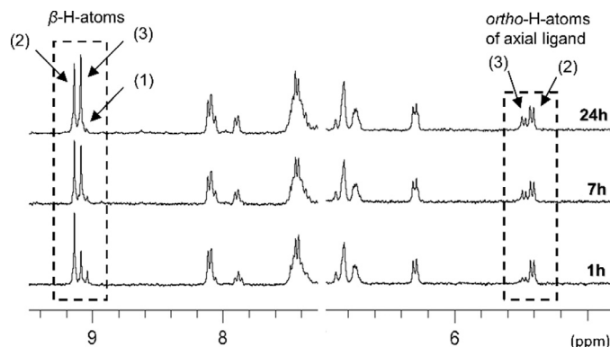
Fig. 2. ^1\text{H} NMR in \text{C}_6\text{D}_6 showing progress of Kocheshkov reaction over reflux time in toluene for the educt ratio of (2):(1)=3:1.
