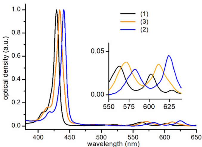
Fig. 6. UVVIS spectra of (1), (2) and (3) in C_6H_6 , inset: detailed spectra of Q-band region.
