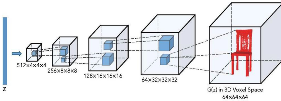
Fig. 1. Image generation /learning with the help of 3D GAN modelling (Wu et al., 2016).
