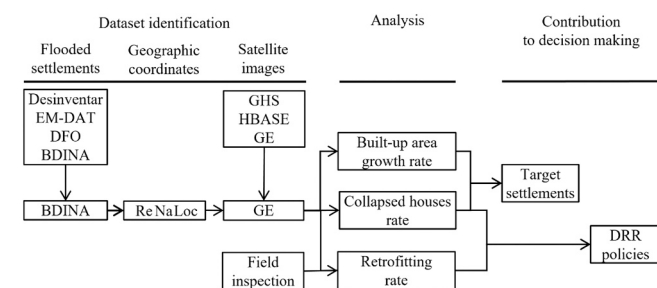
Fig. 2. Analysis flowchart. BDINA- National database on floods, DFO-Dartmouth Flood Observatory, DRR-Disaster risk reduction, GE-Google Earth Pro, GHS-Global Human Settlements dataset, HBASE-Global Human Built-up and Settlement Extent, ReNaLoc-Human settlements national directory.
