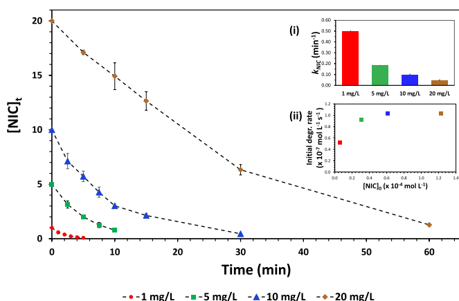
Fig. 1. Effect of concentration on the UV 254 -induced photolysis of nicotine in ultrapure water. Inset graphs: (i) apparent rate constants for each concentration tested and (ii) initial nicotine degradation rates as a function of concentration. Data points are linked with dashed lines to visualize trends. Some error bars are too small to be visible.
