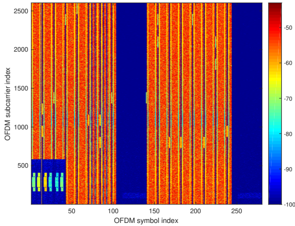
FIGURE 3. Power vs Symbol x Carrier map; the x-axis represents the symbols; the y-axis represents the subcarriers; different colors in the diagram area represent the power; a color map in the diagram header indicates the corresponding power levels in [dBm]; the communication system was forced to give all the resources to only one user.
