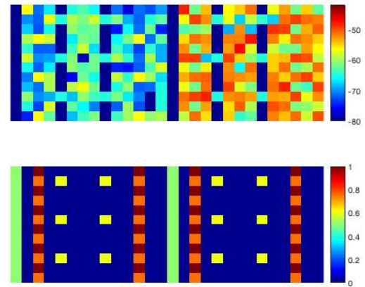
FIGURE 8. An example of two consecutive RBs associated to two different users served by two different data traffic; upper figure: RE power plotted in false colors, from -80 dBm to -40 dBm; lower figure: RBs structure (the different functions of the RE are plotted in false colors according to the scale on the right: CORESET =0.5, PDSCH-DMRS=1 and 0.8, NZP CSI-RS=0.6 and 0.5, ZP CSI-RS=0.2)
