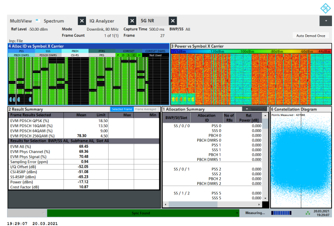
FIGURE 13. An example of VNA output; the Power vs Symbol x Carrier map is drawn in the upper right window; Allocation ID vs Symbol x Carrier is drawn in the upper left window; the Allocation Summary windows reported on the lower windows show various parameters of the measured allocations in a table.
