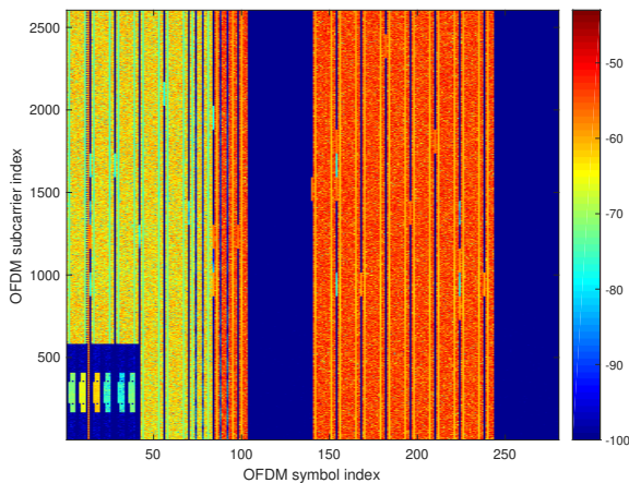
FIGURE 7. Power vs Symbol x Carrier map [dBm]; the communication system was forced to give all the resources to two users served by two different data traffic.
