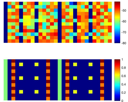
FIGURE 5. An example of two consecutive RBs; in the upper figure the RE power is plotted in false colors, from -80 dBm to -40 dBm; it is possible to note some regular structures; these structures are associated to control signals; in order to identify these structure in the lower figure the different functions of the related REs are plotted in false color according to the scale on the right; COREST are plotted in green (color code 0.5 of the right color scale), PDSCH-DMRS are plotted in red bright and deep red (color codes 1 and 0.8), TRS are colored in yellow (color code=0.6).
