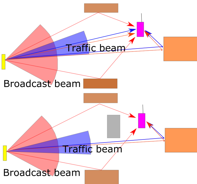
FIGURE 2. Example of LOS communication channel (upper figure) and NLOS communication channel (lower figure); in both cases different paths are associated to data beam and broadcast beam due to the different areas illuminated by the two beams; furthermore, also the paths that are common to broadcast and data beam give different contributions on the interference process since they have different amplitudes and phases according to the (complex, i.e. amplitude and phase) patterns of the data and broadcast antennas; this makes the estimation of the standard uncertainty from pattern data very cumbersome.
