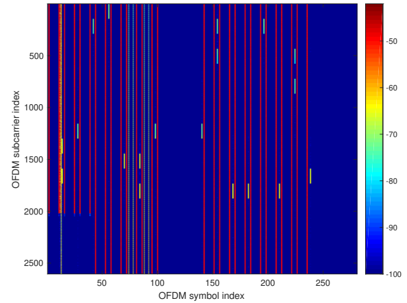
FIGURE 4. Signaling structure in a frame after subtracting SS Blocks and PDSCH REs; the RE power is drawn in false colour according to the scale on the right (in [dBm]).
