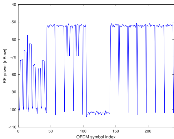
FIGURE 10. Span Zero measurement procedure by Scalar Spectrum Analyzer; the figure shows the power of the REs as obtained from a cut of the frame in a 1 MHz with central bandwidth at the central frequency of the SS Burst.
