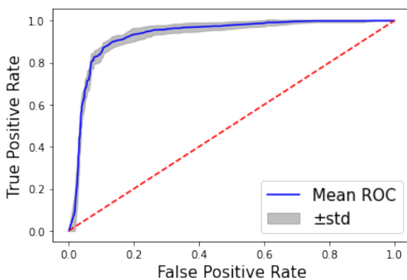
FIGURE 7: ROC curve expressed as an average over 20 iterations. Experiment 2
