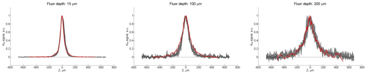
Figure 2. Comparison between experimental K\alpha lineouts (black) and the lineouts obtained from the simulations (red) for flat targets. Fluor depths from left to right are 15, 100 and 200 \mu\text{m} . The range in the experimental data is shown as a gray band.
