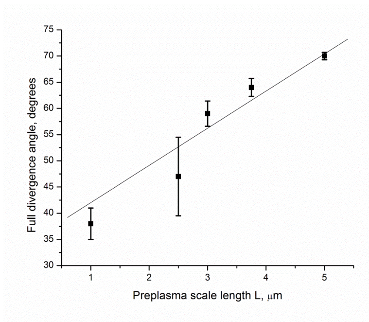
Figure 3. Electron beam divergence vs. pre-plasma scale length for buried cone target simulations. Each point and error bar is derived from the growth of the electron spot size at three different depths. The black curve is a linear fit. Divergence angle increases 7.0^{\circ} \pm 0.6^{\circ} for each 1 \mu\text{m} increase of scale length L.
