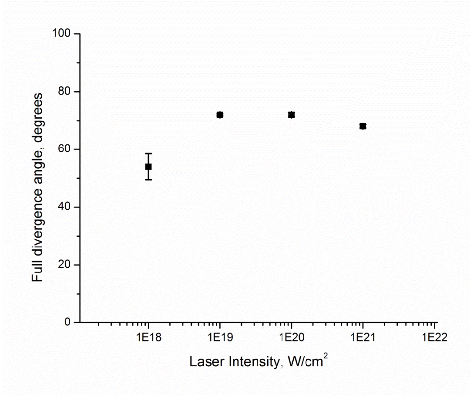
Figure 4. Electron beam divergence vs. laser intensity. The divergence angle was determined by the same method as in Figure 3. Error bars on the graph are from the fitting errors.
