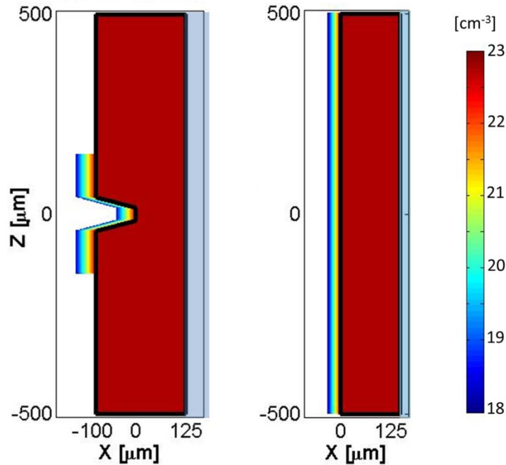
Figure 1. Simulation geometry for the buried cone target (left) and the flat target (right). The black line indicates the solid density contour, the grey line the simulation grid. The color scale on the right shows electron number density in \text{cm}^{-3} (log scale). The laser is incident from the left and focused at the origin. The light blue color represents a region that absorbs electrons (see ref. [15]). Each simulation ran for 10 ps.
