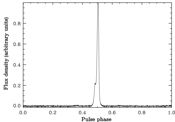
Figure 1. High signal-to-noise profile created by all useable data taken of PSR J1802–2124 at the GBT with the GASP pulsar backend instrument. A noise-free template profile, created by fitting multiple Gaussians to the PSR J1802–2124 pulse profile, was used for timing analysis.
